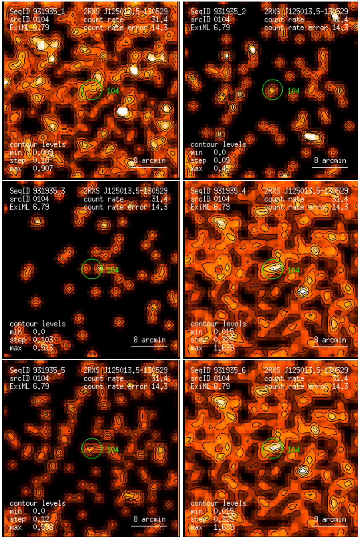
Figure 104: RASS 931935: detection 0104: band rate images, Gaussian filter: (1) PSPC channels 11 – 41, (2) 52 – 90, (3) 91 – 201, (4) 11 – 235, (5) 52 – 201, (6) 11 – 201. Broad band rates in counts/ks. Band rate contour levels in counts/ks/arcmin 2 .
