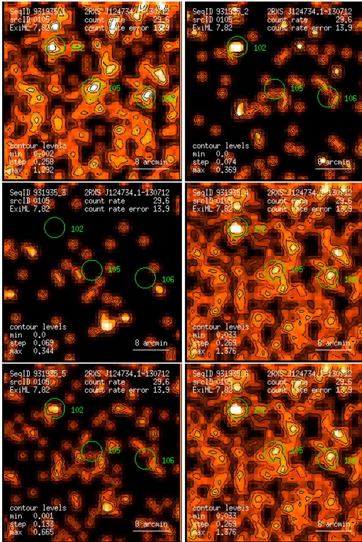
Figure 105: RASS 931935: detection 0105: band rate images, Gaussian filter: (1) PSPC channels 11 – 41, (2) 52 – 90, (3) 91 – 201, (4) 11 – 235, (5) 52 – 201, (6) 11 – 201. Broad band rates in counts/ks. Band rate contour levels in counts/ks/arcmin 2 .
