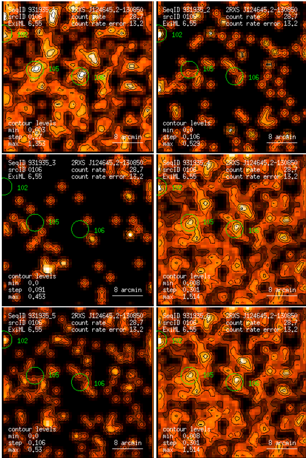
Figure 106: RASS 931935: detection 0106: band rate images, Gaussian filter: (1) PSPC channels 11 – 41, (2) 52 – 90, (3) 91 – 201, (4) 11 – 235, (5) 52 – 201, (6) 11 – 201. Broad band rates in counts/ks. Band rate contour levels in counts/ks/arcmin 2 .
