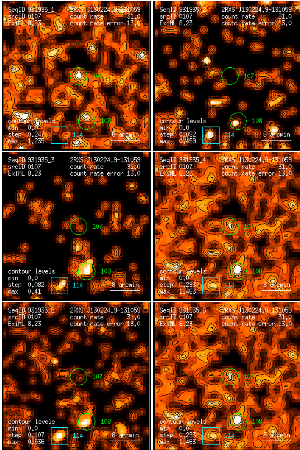
Figure 107: RASS 931935: detection 0107: band rate images, Gaussian filter: (1) PSPC channels 11 – 41, (2) 52 – 90, (3) 91 – 201, (4) 11 – 235, (5) 52 – 201, (6) 11 – 201. Broad band rates in counts/ks. Band rate contour levels in counts/ks/arcmin 2 .
