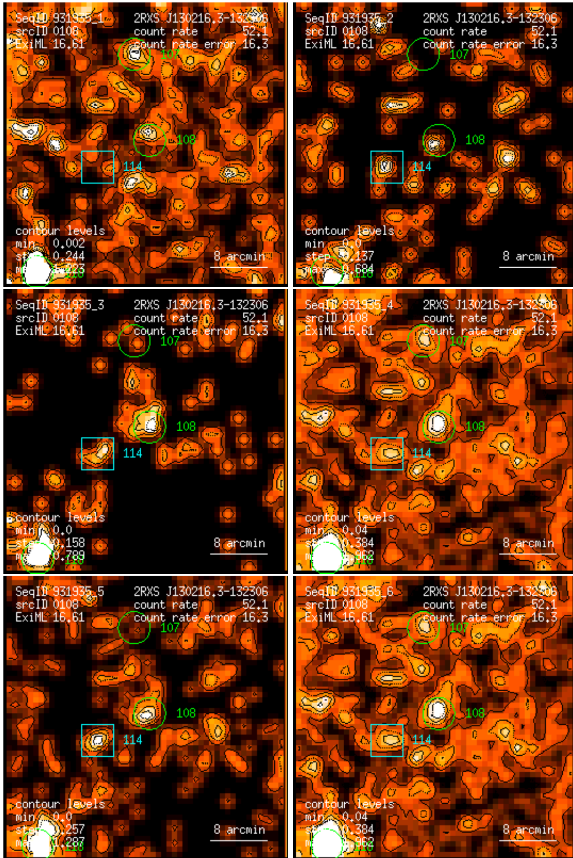
Figure 108: RASS 931935: detection 0108: band rate images, Gaussian filter: (1) PSPC channels 11 – 41, (2) 52 – 90, (3) 91 – 201, (4) 11 – 235, (5) 52 – 201, (6) 11 – 201. Broad band rates in counts/ks. Band rate contour levels in counts/ks/arcmin 2 .
