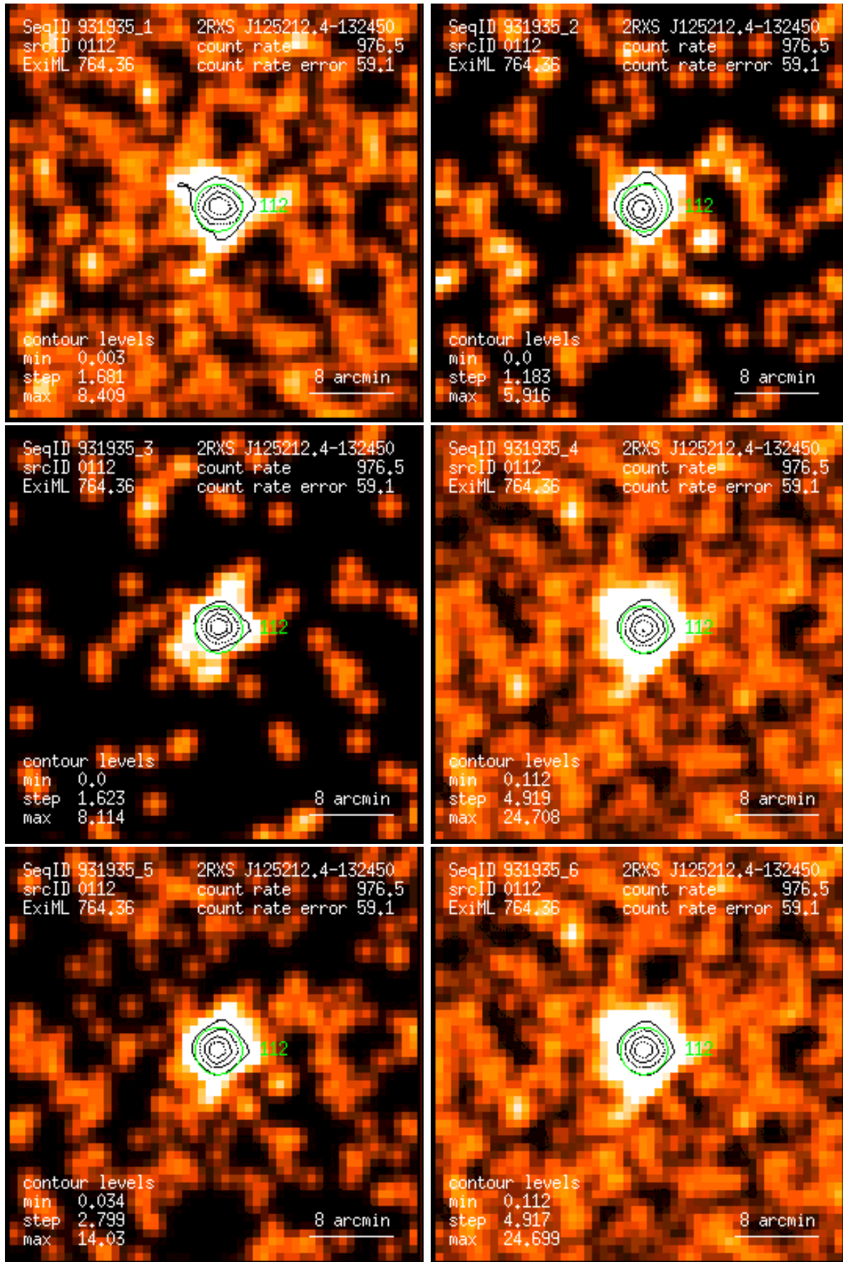
Figure 112: RASS 931935: detection 0112: band rate images, Gaussian filter: (1) PSPC channels 11 – 41, (2) 52 – 90, (3) 91 – 201, (4) 11 – 235, (5) 52 – 201, (6) 11 – 201. Broad band rates in counts/ks. Band rate contour levels in counts/ks/arcmin 2 .
