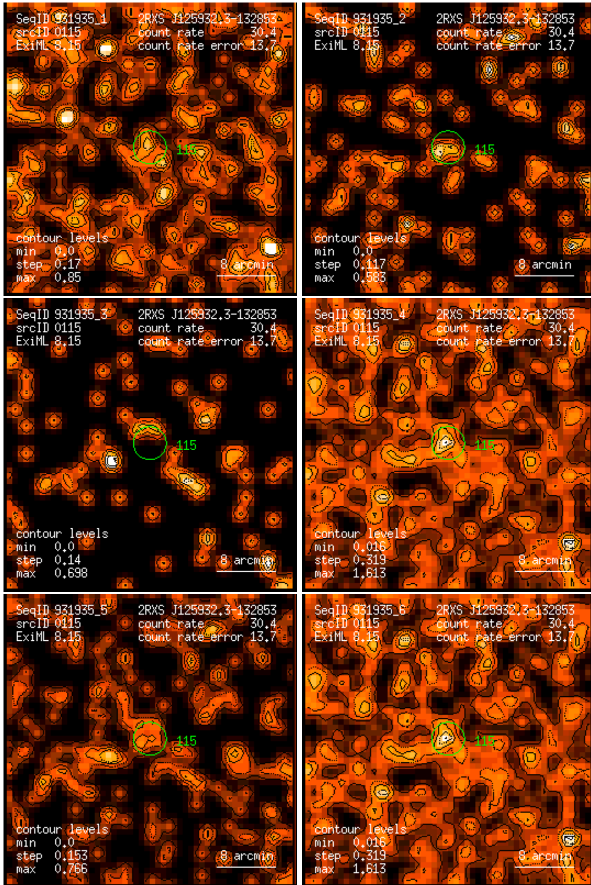
Figure 115: RASS 931935: detection 0115: band rate images, Gaussian filter: (1) PSPC channels 11 – 41, (2) 52 – 90, (3) 91 – 201, (4) 11 – 235, (5) 52 – 201, (6) 11 – 201. Broad band rates in counts/ks. Band rate contour levels in counts/ks/arcmin 2 .
