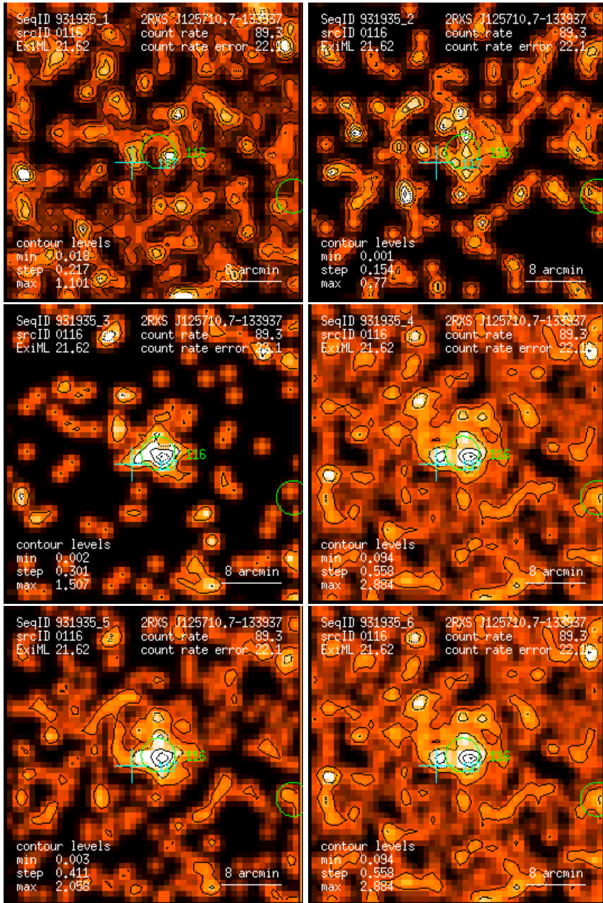
Figure 116: RASS 931935: detection 0116: band rate images, Gaussian filter: (1) PSPC channels 11 – 41, (2) 52 – 90, (3) 91 – 201, (4) 11 – 235, (5) 52 – 201, (6) 11 – 201. Broad band rates in counts/ks. Band rate contour levels in counts/ks/arcmin 2 .
