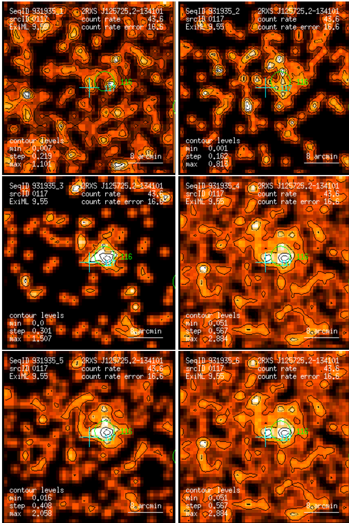
Figure 117: RASS 931935: detection 0117: band rate images, Gaussian filter: (1) PSPC channels 11 – 41, (2) 52 – 90, (3) 91 – 201, (4) 11 – 235, (5) 52 – 201, (6) 11 – 201. Broad band rates in counts/ks. Band rate contour levels in counts/ks/arcmin 2 .
