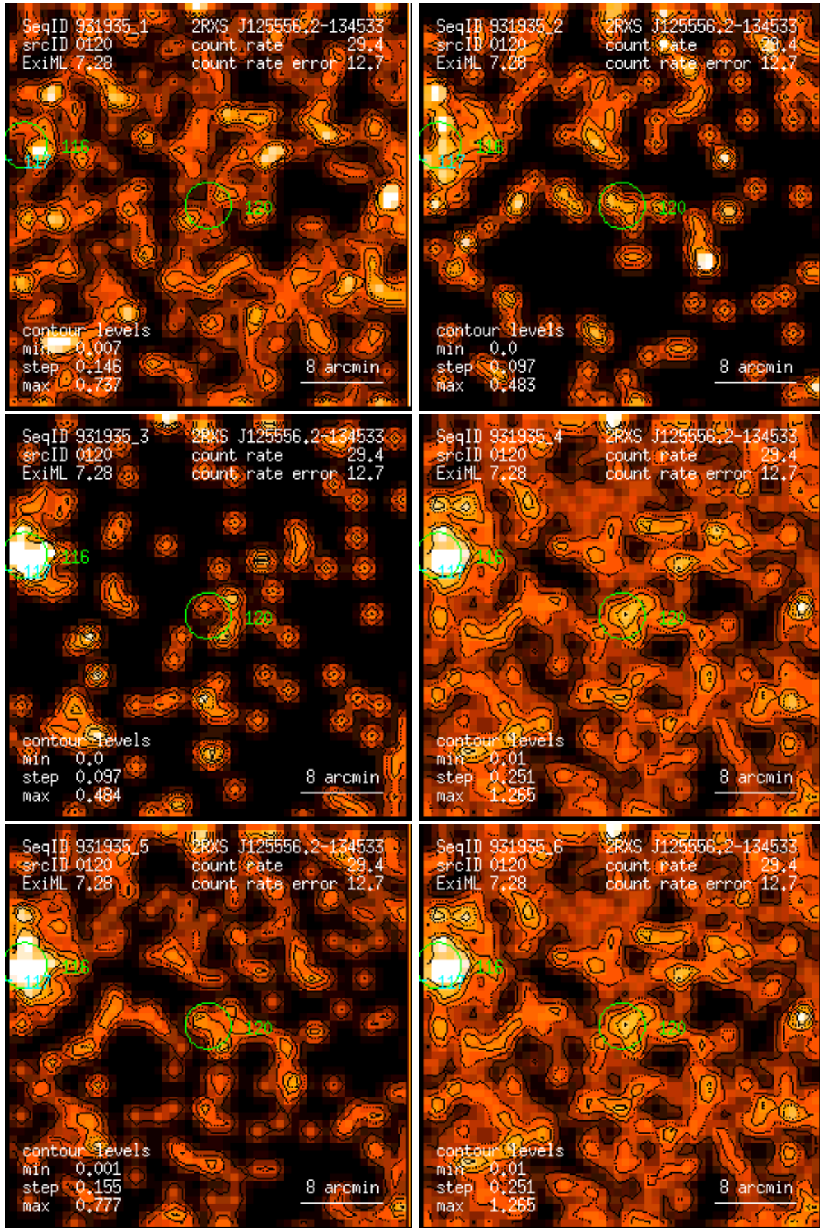
Figure 120: RASS 931935: detection 0120: band rate images, Gaussian filter: (1) PSPC channels 11 – 41, (2) 52 – 90, (3) 91 – 201, (4) 11 – 235, (5) 52 – 201, (6) 11 – 201. Broad band rates in counts/ks. Band rate contour levels in counts/ks/arcmin 2 .
