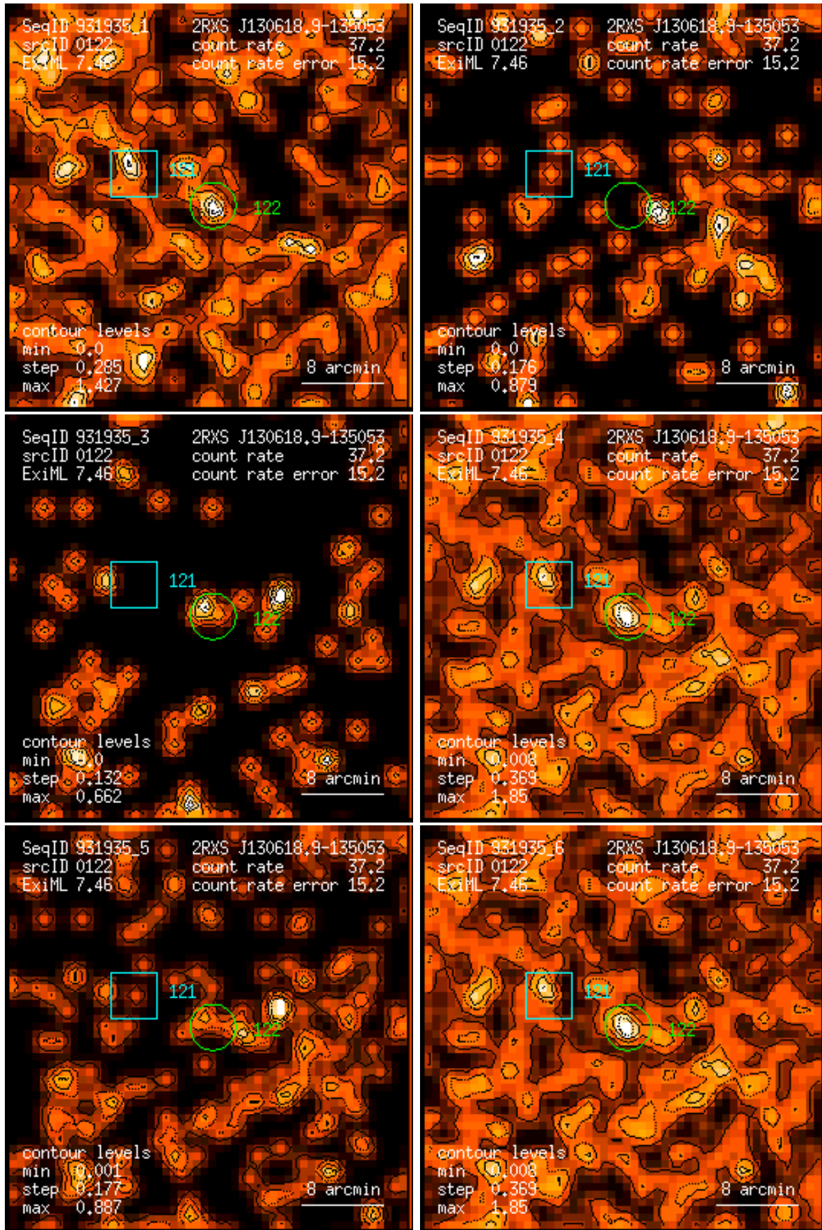
Figure 122: RASS 931935: detection 0122: band rate images, Gaussian filter: (1) PSPC channels 11 – 41, (2) 52 – 90, (3) 91 – 201, (4) 11 – 235, (5) 52 – 201, (6) 11 – 201. Broad band rates in counts/ks. Band rate contour levels in counts/ks/arcmin 2 .
