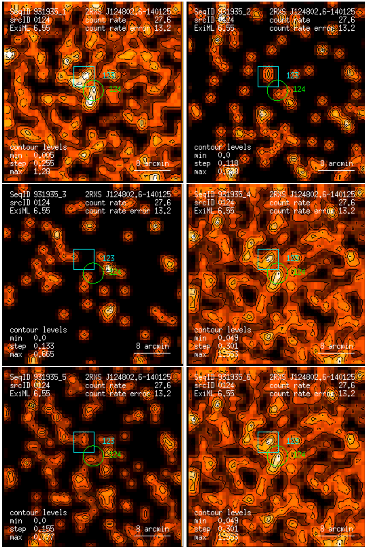
Figure 124: RASS 931935: detection 0124: band rate images, Gaussian filter: (1) PSPC channels 11 – 41, (2) 52 – 90, (3) 91 – 201, (4) 11 – 235, (5) 52 – 201, (6) 11 – 201. Broad band rates in counts/ks. Band rate contour levels in counts/ks/arcmin 2 .
