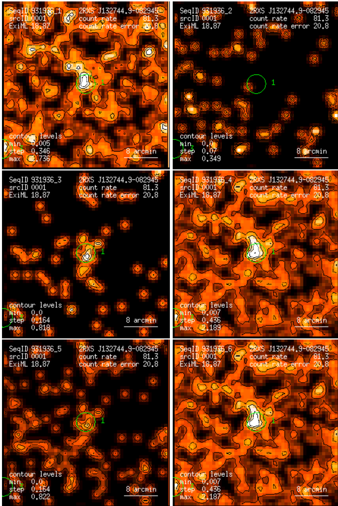
Figure 1: RASS 931936: detection 0001: band rate images, Gaussian filter: (1) PSPC channels 11 – 41, (2) 52 – 90, (3) 91 – 201, (4) 11 – 235, (5) 52 – 201, (6) 11 – 201. Broad band rates in counts/ks. Band rate contour levels in counts/ks/arcmin 2 .
