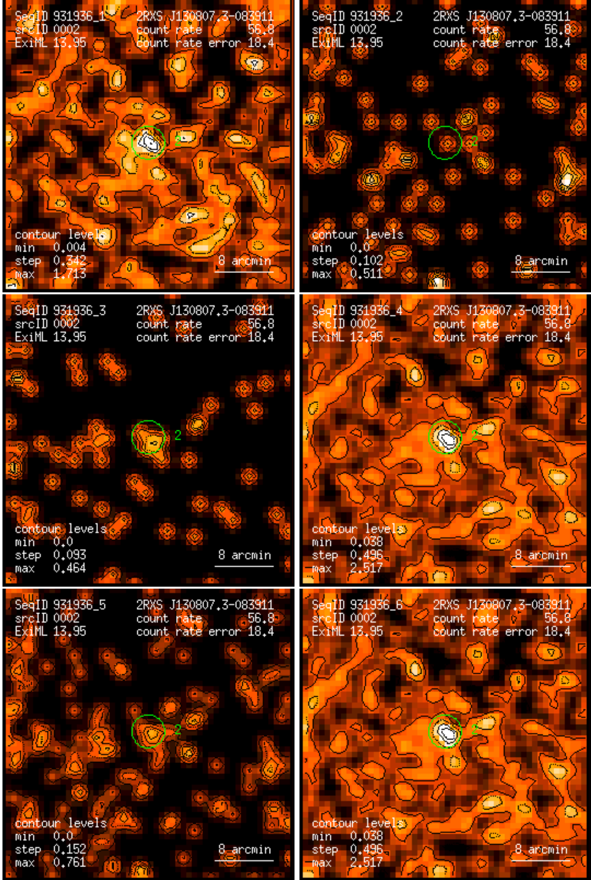
Figure 2: RASS 931936: detection 0002: band rate images, Gaussian filter: (1) PSPC channels 11 – 41, (2) 52 – 90, (3) 91 – 201, (4) 11 – 235, (5) 52 – 201, (6) 11 – 201. Broad band rates in counts/ks. Band rate contour levels in counts/ks/arcmin 2 .
