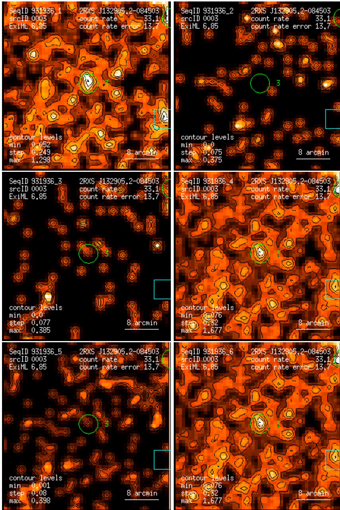
Figure 3: RASS 931936: detection 0003: band rate images, Gaussian filter: (1) PSPC channels 11 – 41, (2) 52 – 90, (3) 91 – 201, (4) 11 – 235, (5) 52 – 201, (6) 11 – 201. Broad band rates in counts/ks. Band rate contour levels in counts/ks/arcmin 2 .
