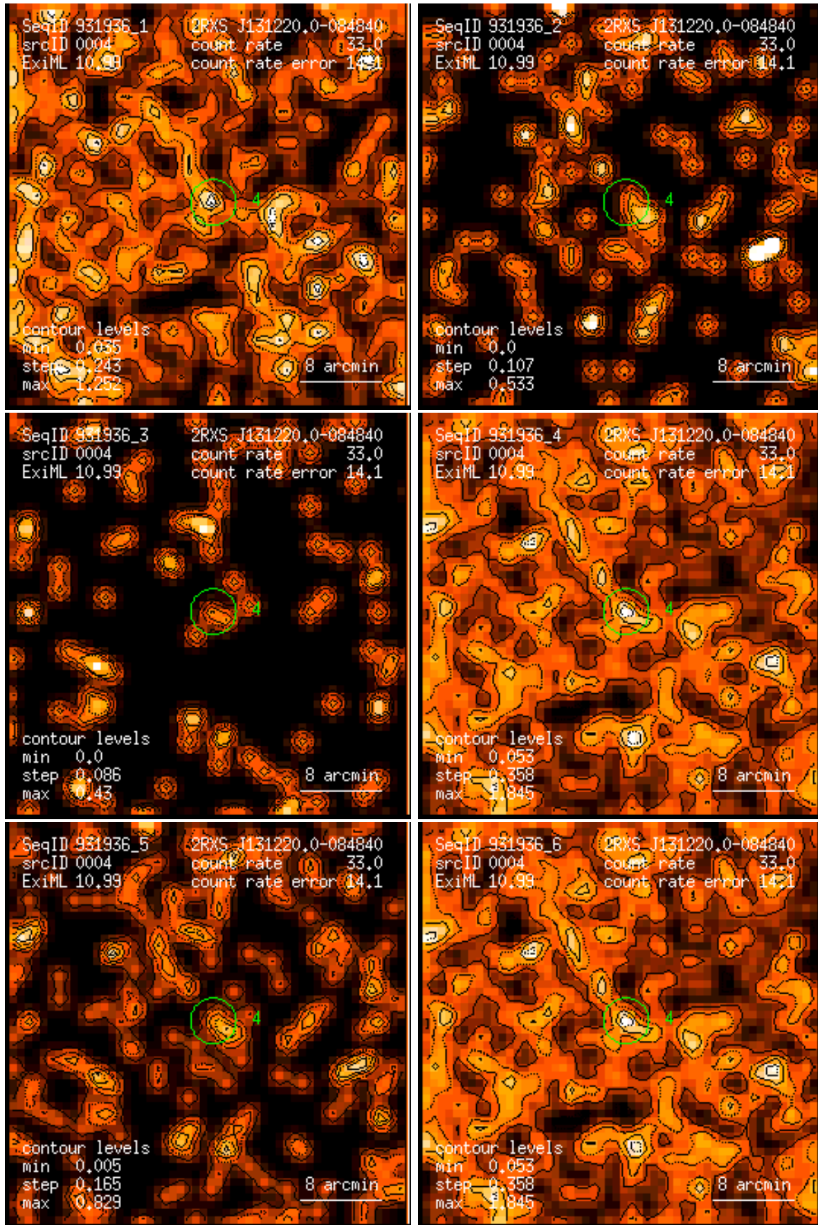
Figure 4: RASS 931936: detection 0004: band rate images, Gaussian filter: (1) PSPC channels 11 – 41, (2) 52 – 90, (3) 91 – 201, (4) 11 – 235, (5) 52 – 201, (6) 11 – 201. Broad band rates in counts/ks. Band rate contour levels in counts/ks/arcmin 2 .
