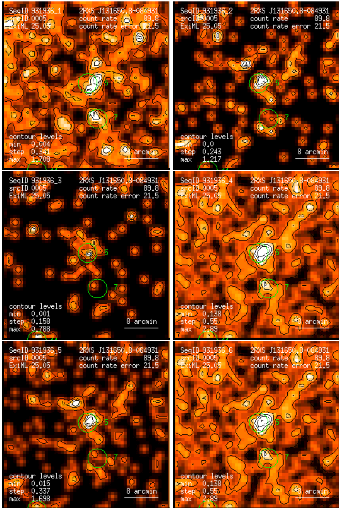
Figure 5: RASS 931936: detection 0005: band rate images, Gaussian filter: (1) PSPC channels 11 – 41, (2) 52 – 90, (3) 91 – 201, (4) 11 – 235, (5) 52 – 201, (6) 11 – 201. Broad band rates in counts/ks. Band rate contour levels in counts/ks/arcmin 2 .
