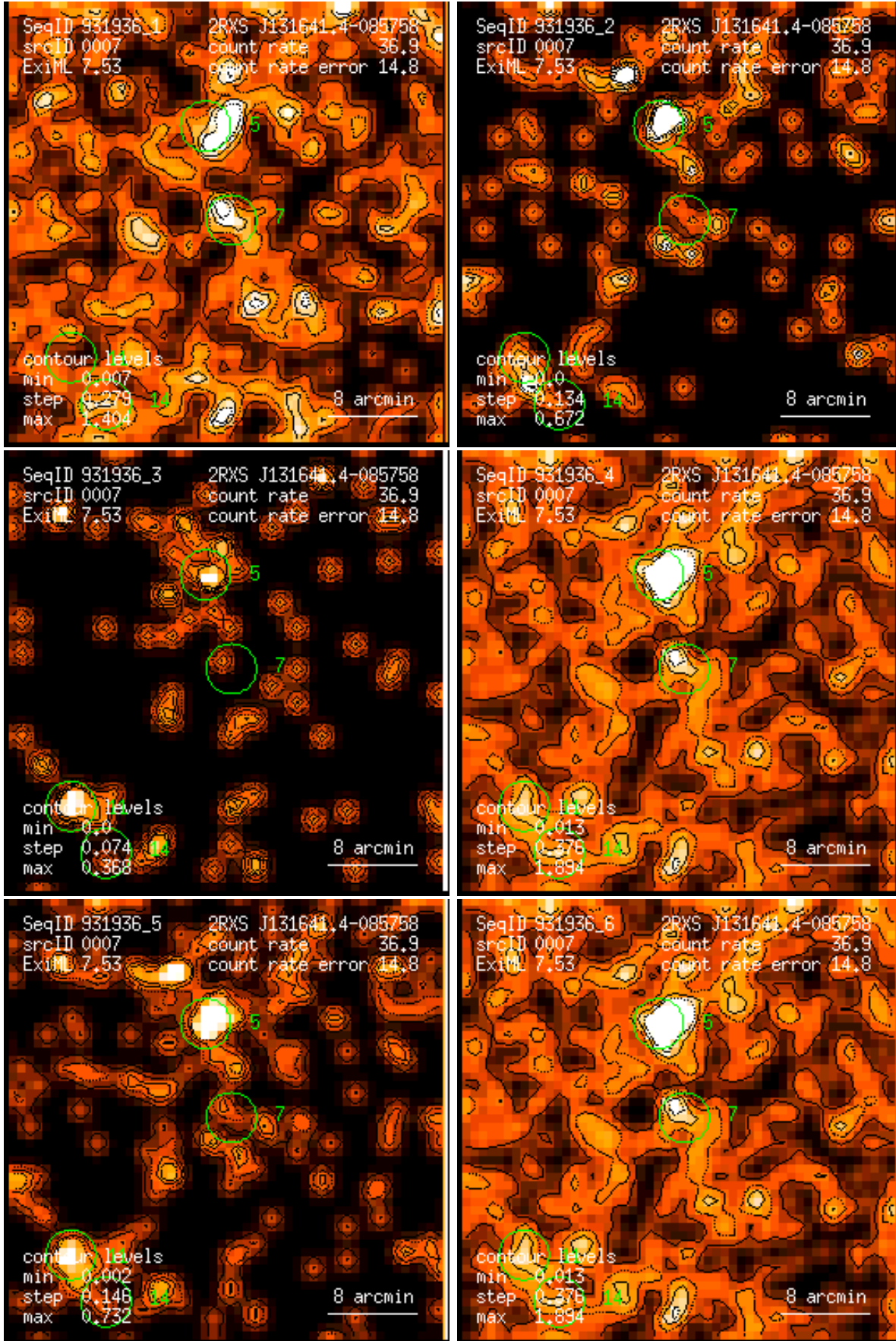
Figure 7: RASS 931936: detection 0007: band rate images, Gaussian filter: (1) PSPC channels 11 – 41, (2) 52 – 90, (3) 91 – 201, (4) 11 – 235, (5) 52 – 201, (6) 11 – 201. Broad band rates in counts/ks. Band rate contour levels in counts/ks/arcmin 2 .
