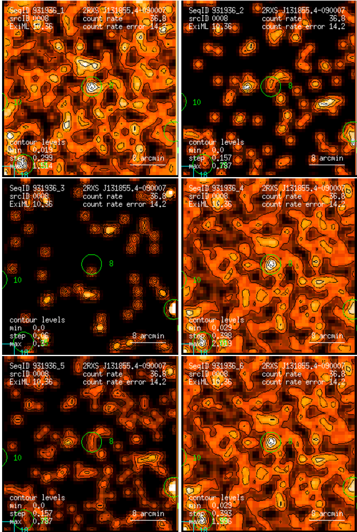
Figure 8: RASS 931936: detection 0008: band rate images, Gaussian filter: (1) PSPC channels 11 – 41, (2) 52 – 90, (3) 91 – 201, (4) 11 – 235, (5) 52 – 201, (6) 11 – 201. Broad band rates in counts/ks. Band rate contour levels in counts/ks/arcmin 2 .
