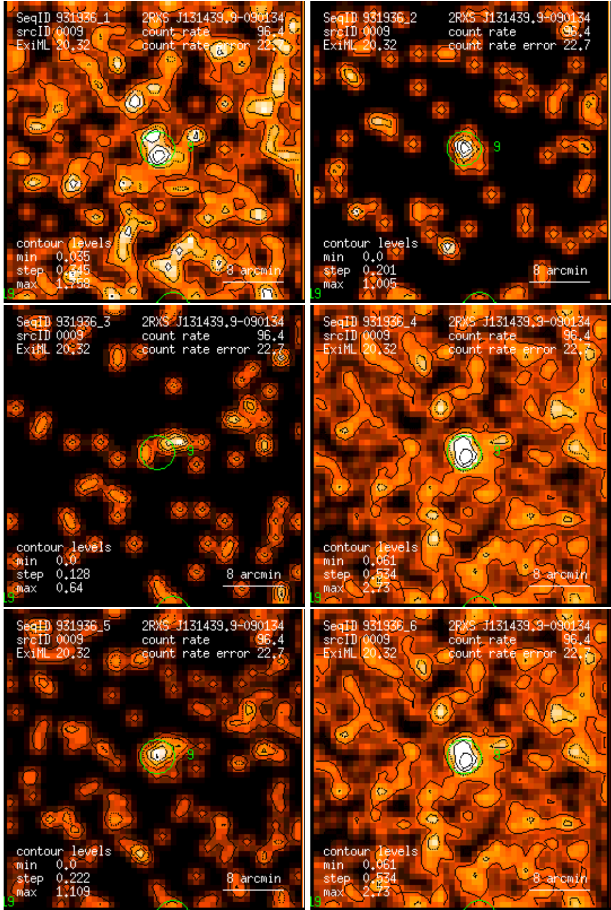
Figure 9: RASS 931936: detection 0009: band rate images, Gaussian filter: (1) PSPC channels 11 – 41, (2) 52 – 90, (3) 91 – 201, (4) 11 – 235, (5) 52 – 201, (6) 11 – 201. Broad band rates in counts/ks. Band rate contour levels in counts/ks/arcmin 2 .
