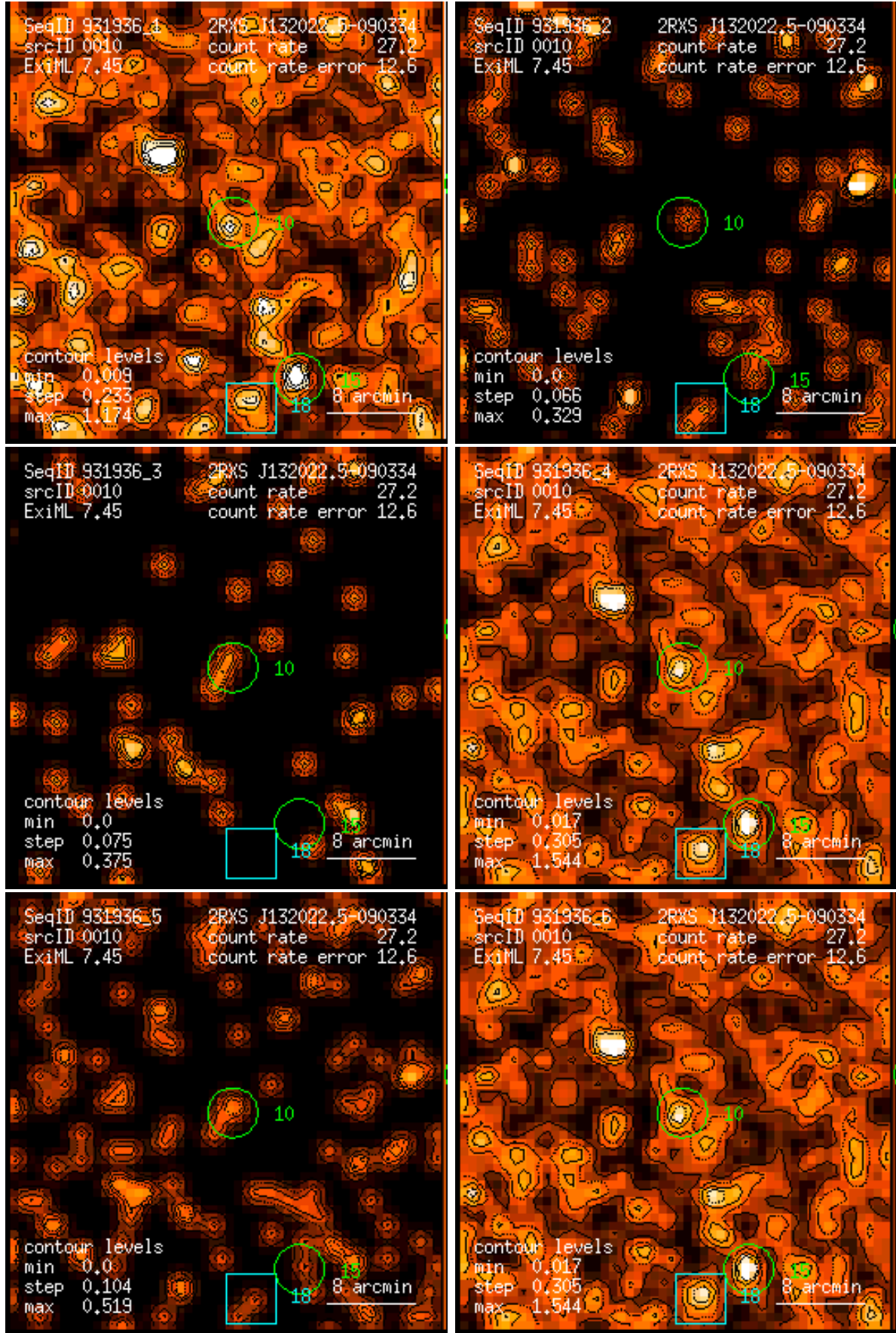
Figure 10: RASS 931936: detection 0010: band rate images, Gaussian filter: (1) PSPC channels 11 – 41, (2) 52 – 90, (3) 91 – 201, (4) 11 – 235, (5) 52 – 201, (6) 11 – 201. Broad band rates in counts/ks. Band rate contour levels in counts/ks/arcmin 2 .
