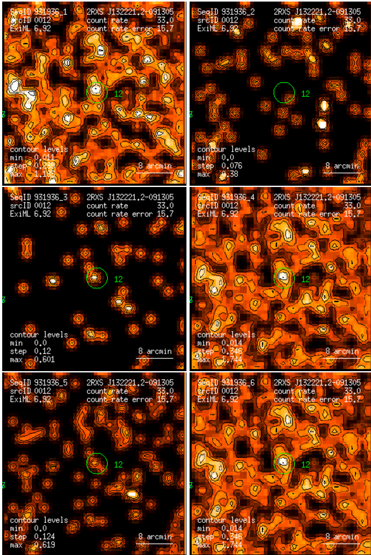
Figure 12: RASS 931936: detection 0012: band rate images, Gaussian filter: (1) PSPC channels 11 – 41, (2) 52 – 90, (3) 91 – 201, (4) 11 – 235, (5) 52 – 201, (6) 11 – 201. Broad band rates in counts/ks. Band rate contour levels in counts/ks/arcmin 2 .
