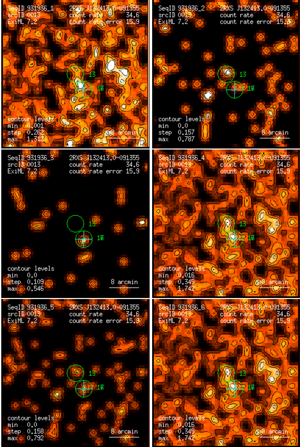
Figure 13: RASS 931936: detection 0013: band rate images, Gaussian filter: (1) PSPC channels 11 – 41, (2) 52 – 90, (3) 91 – 201, (4) 11 – 235, (5) 52 – 201, (6) 11 – 201. Broad band rates in counts/ks. Band rate contour levels in counts/ks/arcmin 2 .
