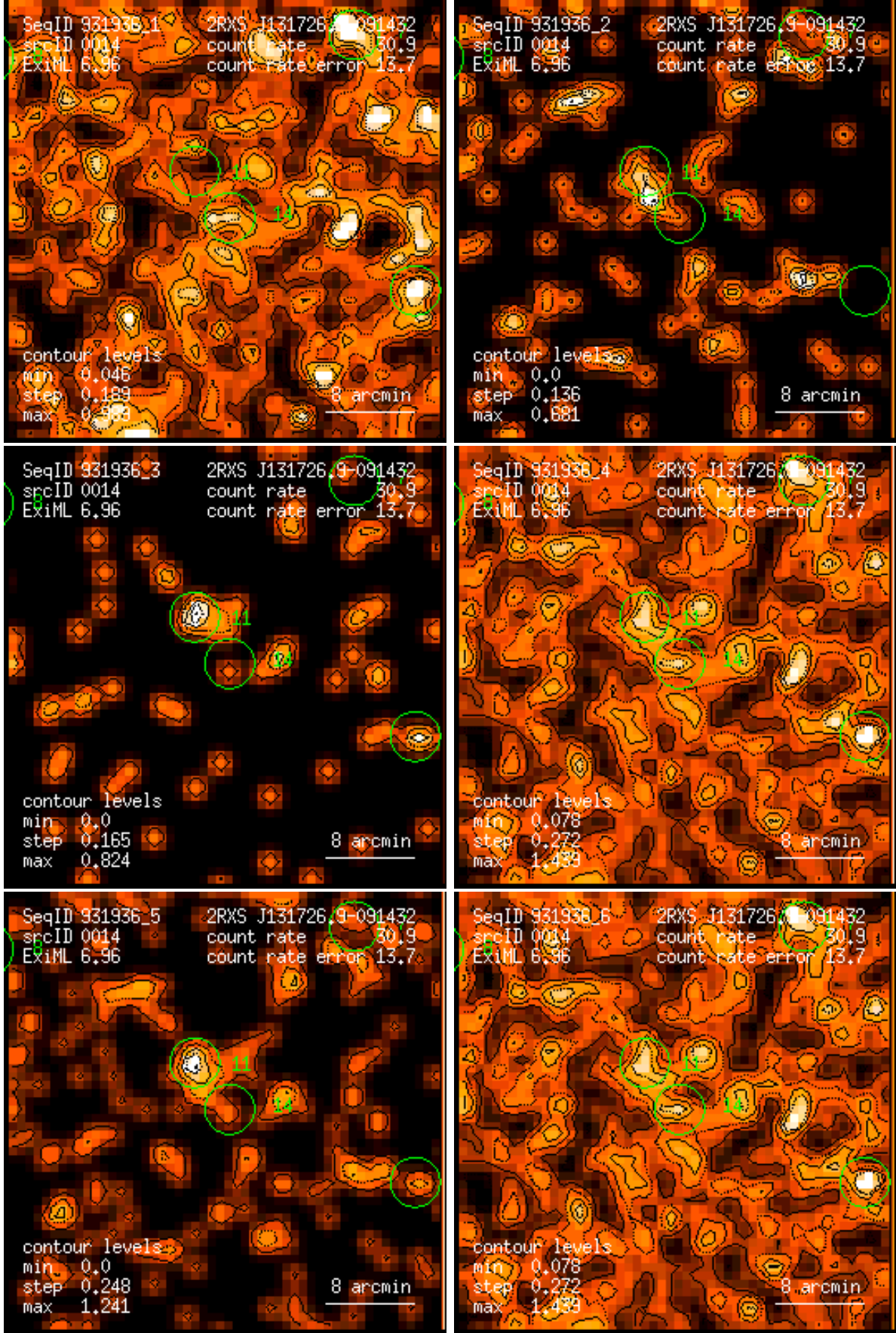
Figure 14: RASS 931936: detection 0014: band rate images, Gaussian filter: (1) PSPC channels 11 – 41, (2) 52 – 90, (3) 91 – 201, (4) 11 – 235, (5) 52 – 201, (6) 11 – 201. Broad band rates in counts/ks. Band rate contour levels in counts/ks/arcmin 2 .
