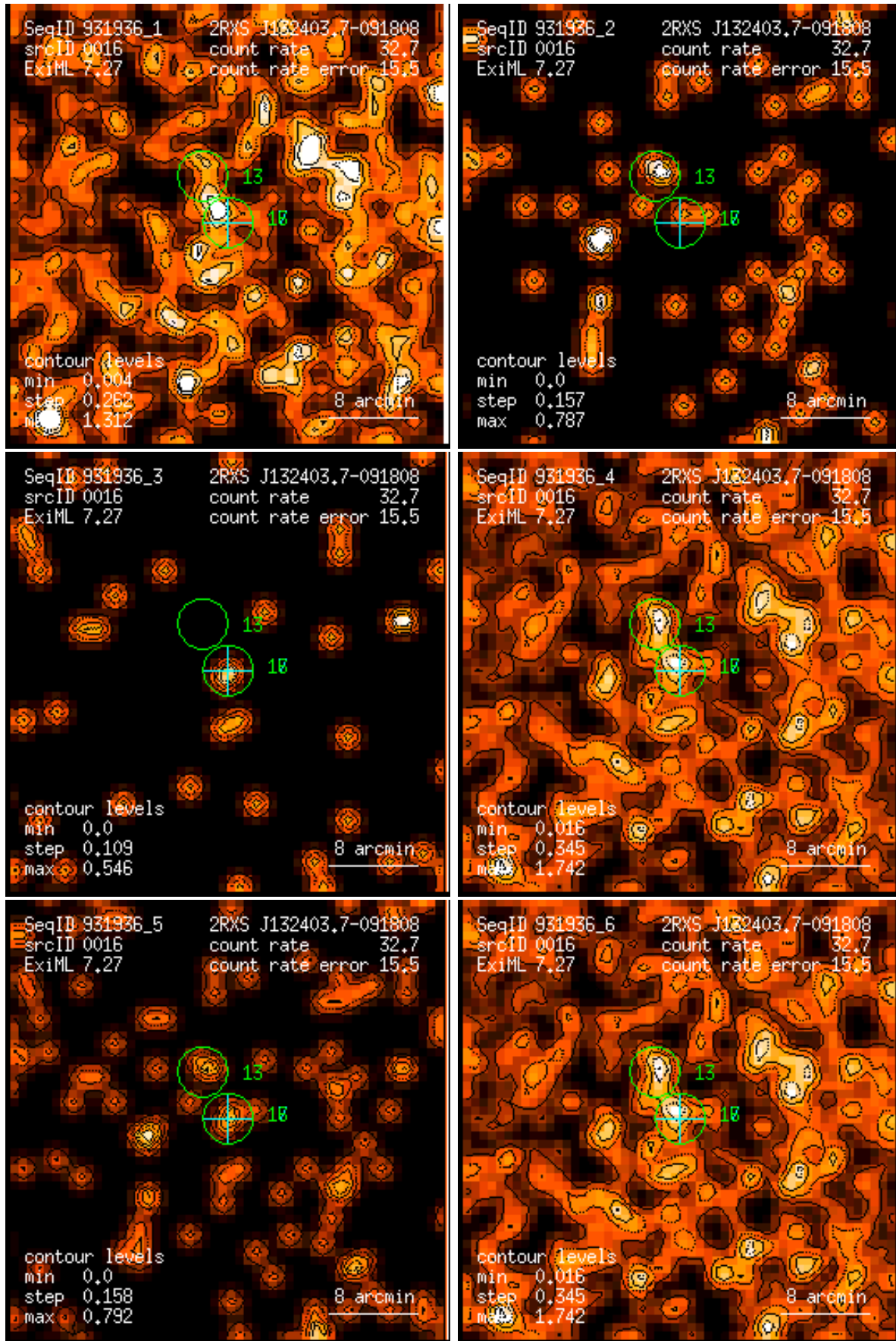
Figure 16: RASS 931936: detection 0016: band rate images, Gaussian filter: (1) PSPC channels 11 – 41, (2) 52 – 90, (3) 91 – 201, (4) 11 – 235, (5) 52 – 201, (6) 11 – 201. Broad band rates in counts/ks. Band rate contour levels in counts/ks/arcmin 2 .
