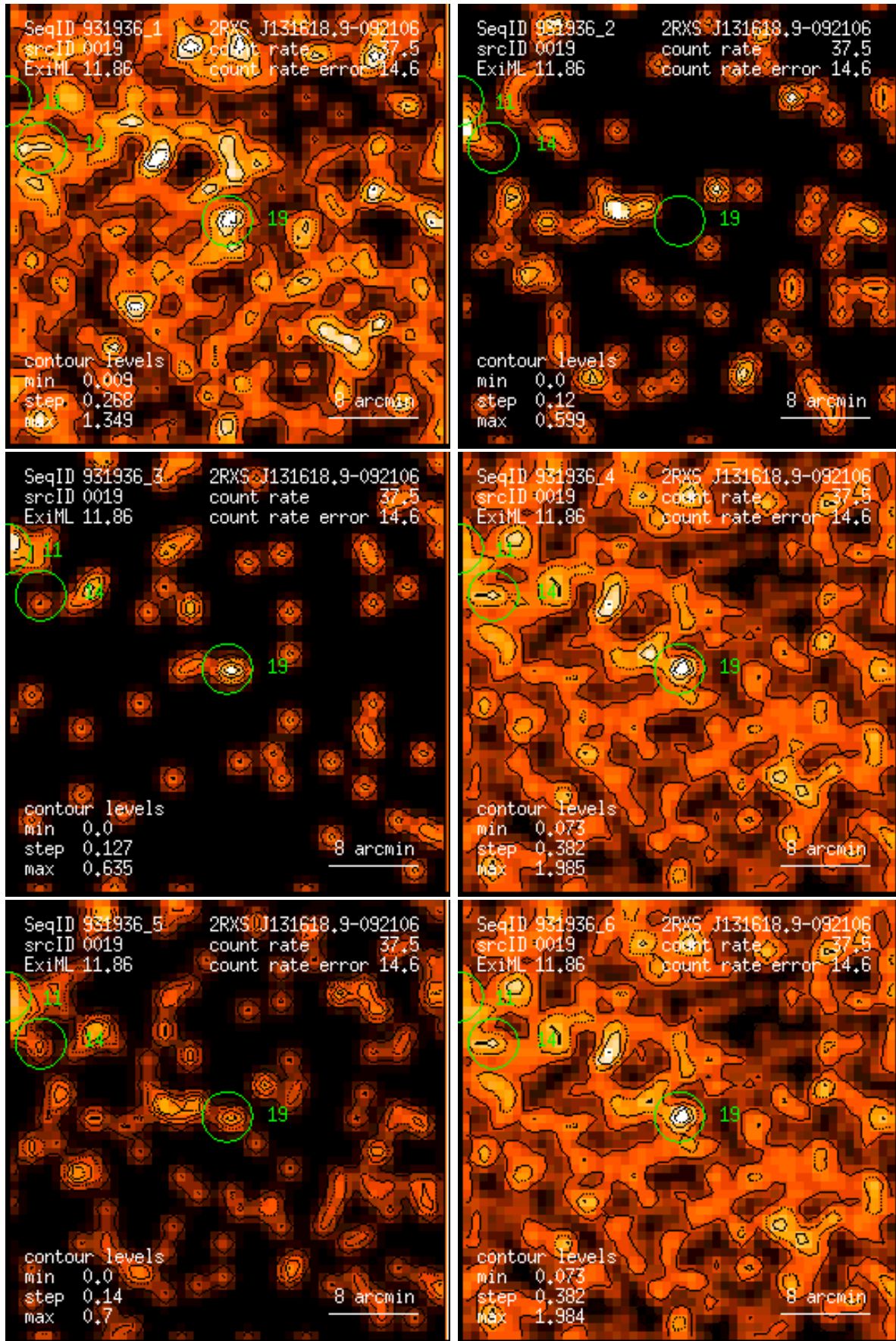
Figure 19: RASS 931936: detection 0019: band rate images, Gaussian filter: (1) PSPC channels 11 – 41, (2) 52 – 90, (3) 91 – 201, (4) 11 – 235, (5) 52 – 201, (6) 11 – 201. Broad band rates in counts/ks. Band rate contour levels in counts/ks/arcmin 2 .
