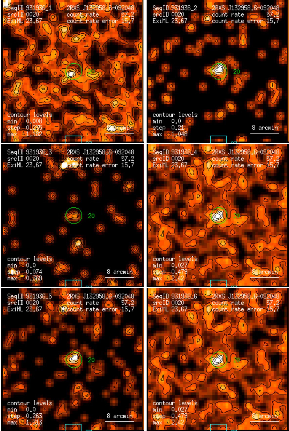
Figure 20: RASS 931936: detection 0020: band rate images, Gaussian filter: (1) PSPC channels 11 – 41, (2) 52 – 90, (3) 91 – 201, (4) 11 – 235, (5) 52 – 201, (6) 11 – 201. Broad band rates in counts/ks. Band rate contour levels in counts/ks/arcmin 2 .
