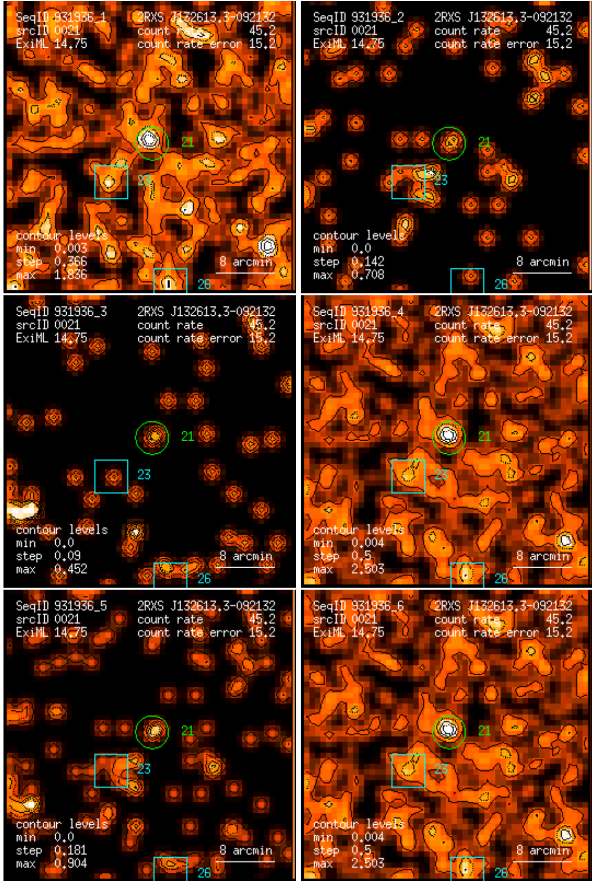
Figure 21: RASS 931936: detection 0021: band rate images, Gaussian filter: (1) PSPC channels 11 – 41, (2) 52 – 90, (3) 91 – 201, (4) 11 – 235, (5) 52 – 201, (6) 11 – 201. Broad band rates in counts/ks. Band rate contour levels in counts/ks/arcmin 2 .
