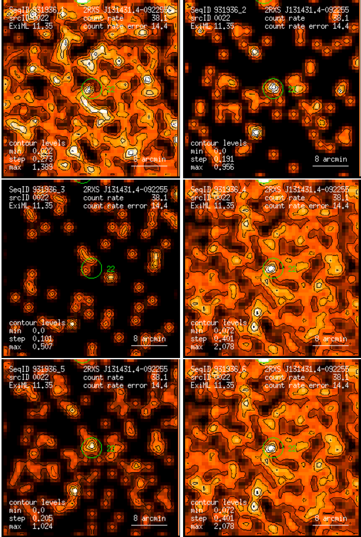
Figure 22: RASS 931936: detection 0022: band rate images, Gaussian filter: (1) PSPC channels 11 – 41, (2) 52 – 90, (3) 91 – 201, (4) 11 – 235, (5) 52 – 201, (6) 11 – 201. Broad band rates in counts/ks. Band rate contour levels in counts/ks/arcmin 2 .
