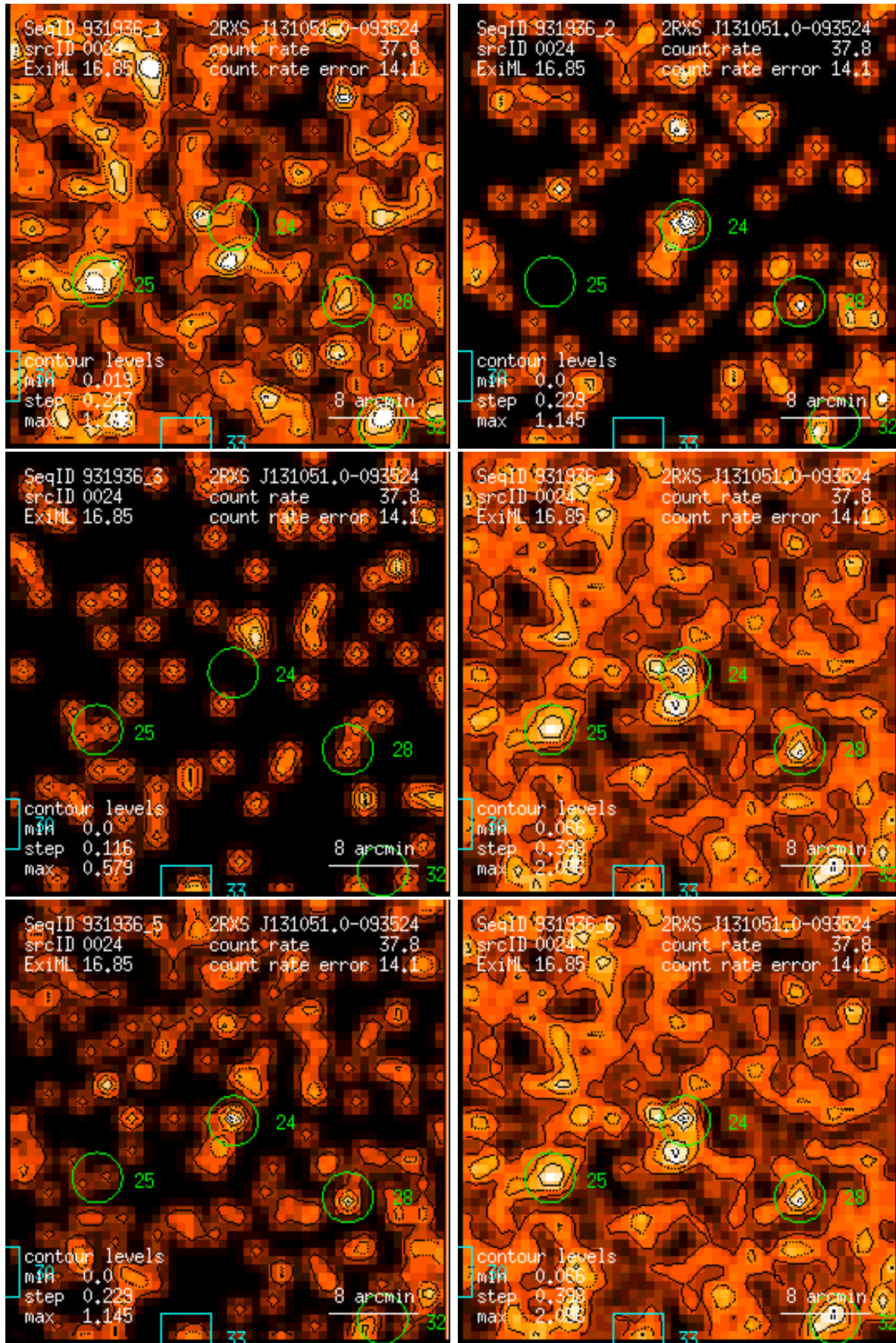
Figure 24: RASS 931936: detection 0024: band rate images, Gaussian filter: (1) PSPC channels 11 – 41, (2) 52 – 90, (3) 91 – 201, (4) 11 – 235, (5) 52 – 201, (6) 11 – 201. Broad band rates in counts/ks. Band rate contour levels in counts/ks/arcmin 2 .
