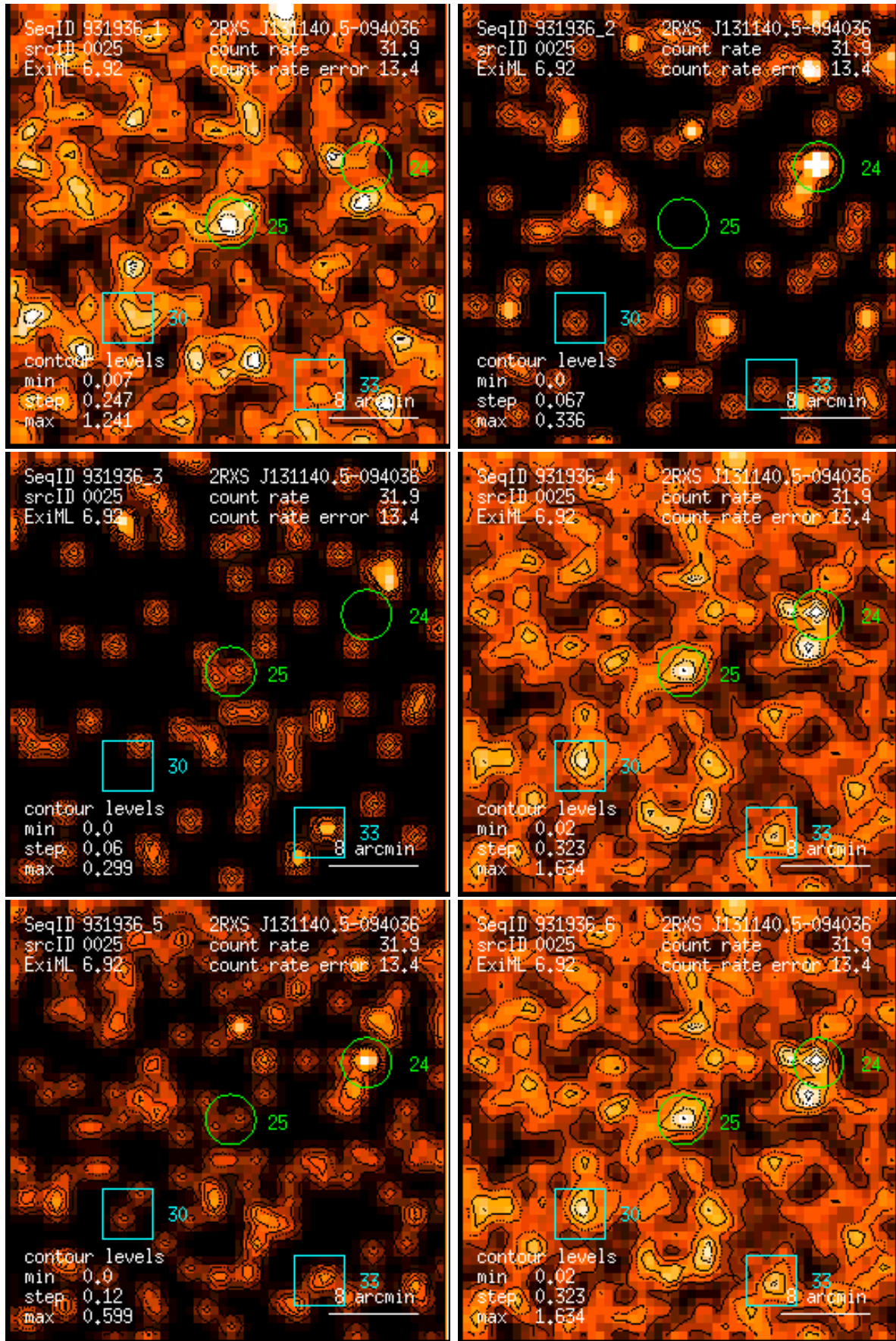
Figure 25: RASS 931936: detection 0025: band rate images, Gaussian filter: (1) PSPC channels 11 – 41, (2) 52 – 90, (3) 91 – 201, (4) 11 – 235, (5) 52 – 201, (6) 11 – 201. Broad band rates in counts/ks. Band rate contour levels in counts/ks/arcmin 2 .
