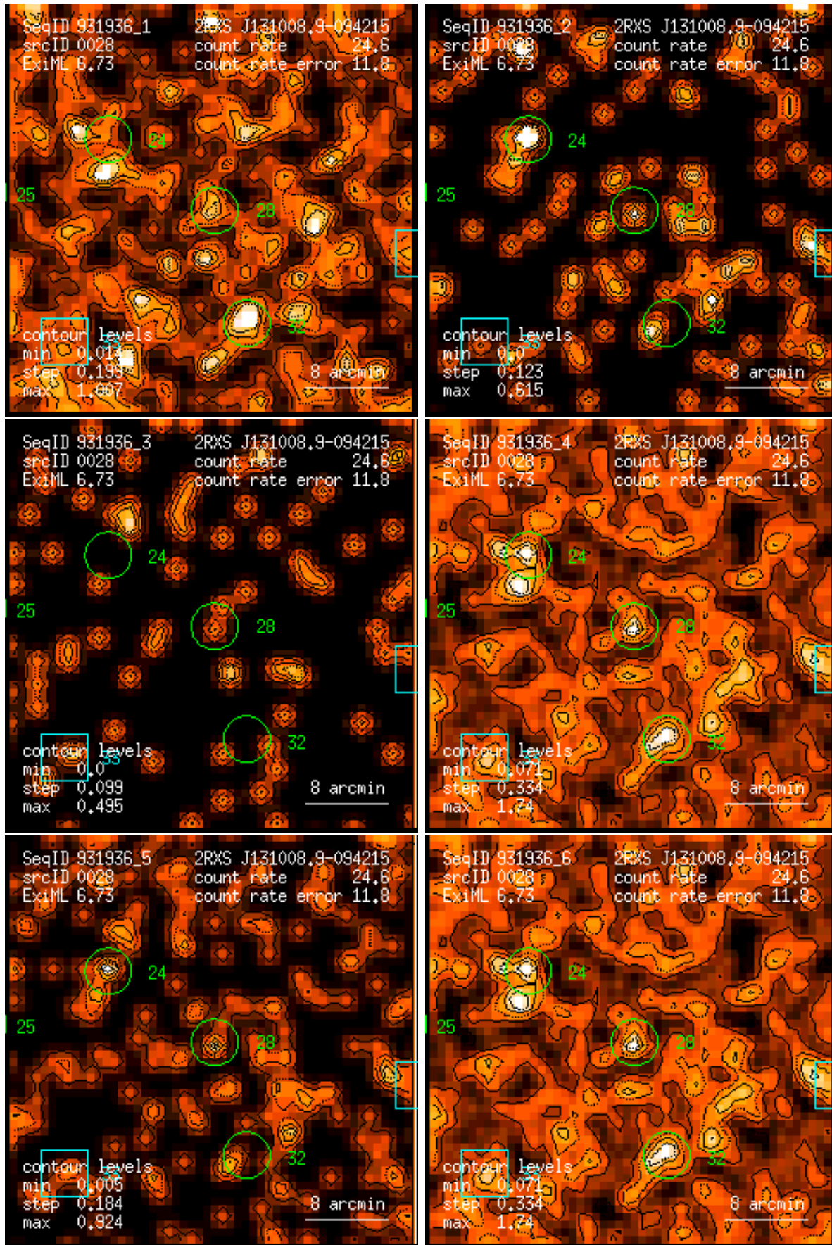
Figure 28: RASS 931936: detection 0028: band rate images, Gaussian filter: (1) PSPC channels 11 – 41, (2) 52 – 90, (3) 91 – 201, (4) 11 – 235, (5) 52 – 201, (6) 11 – 201. Broad band rates in counts/ks. Band rate contour levels in counts/ks/arcmin 2 .
