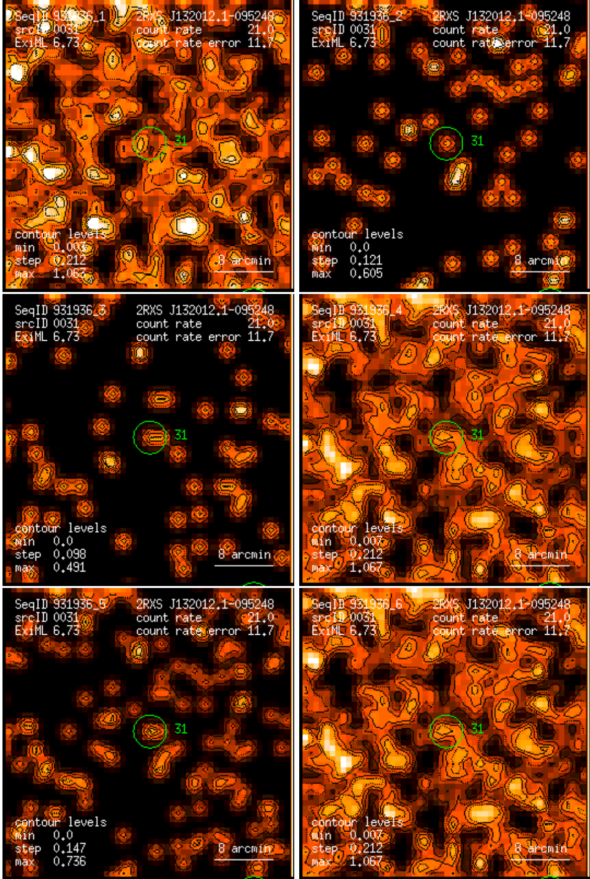
Figure 31: RASS 931936: detection 0031: band rate images, Gaussian filter: (1) PSPC channels 11 – 41, (2) 52 – 90, (3) 91 – 201, (4) 11 – 235, (5) 52 – 201, (6) 11 – 201. Broad band rates in counts/ks. Band rate contour levels in counts/ks/arcmin 2 .
