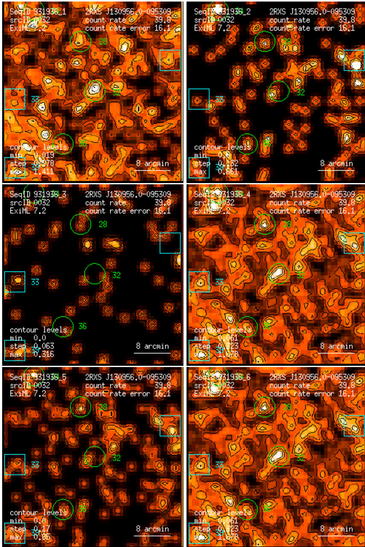
Figure 32: RASS 931936: detection 0032: band rate images, Gaussian filter: (1) PSPC channels 11 – 41, (2) 52 – 90, (3) 91 – 201, (4) 11 – 235, (5) 52 – 201, (6) 11 – 201. Broad band rates in counts/ks. Band rate contour levels in counts/ks/arcmin 2 .
