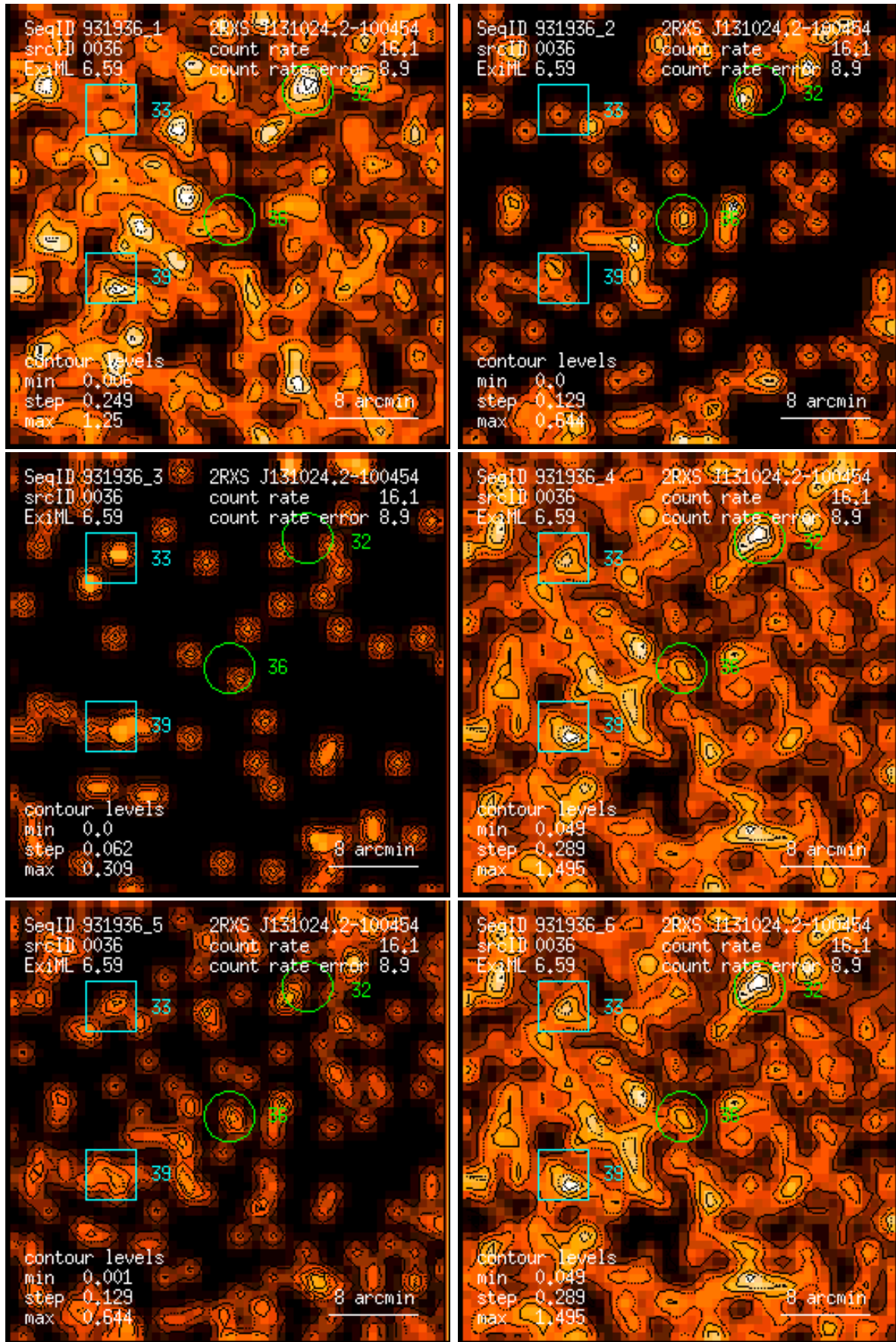
Figure 36: RASS 931936: detection 0036: band rate images, Gaussian filter: (1) PSPC channels 11 – 41, (2) 52 – 90, (3) 91 – 201, (4) 11 – 235, (5) 52 – 201, (6) 11 – 201. Broad band rates in counts/ks. Band rate contour levels in counts/ks/arcmin 2 .
