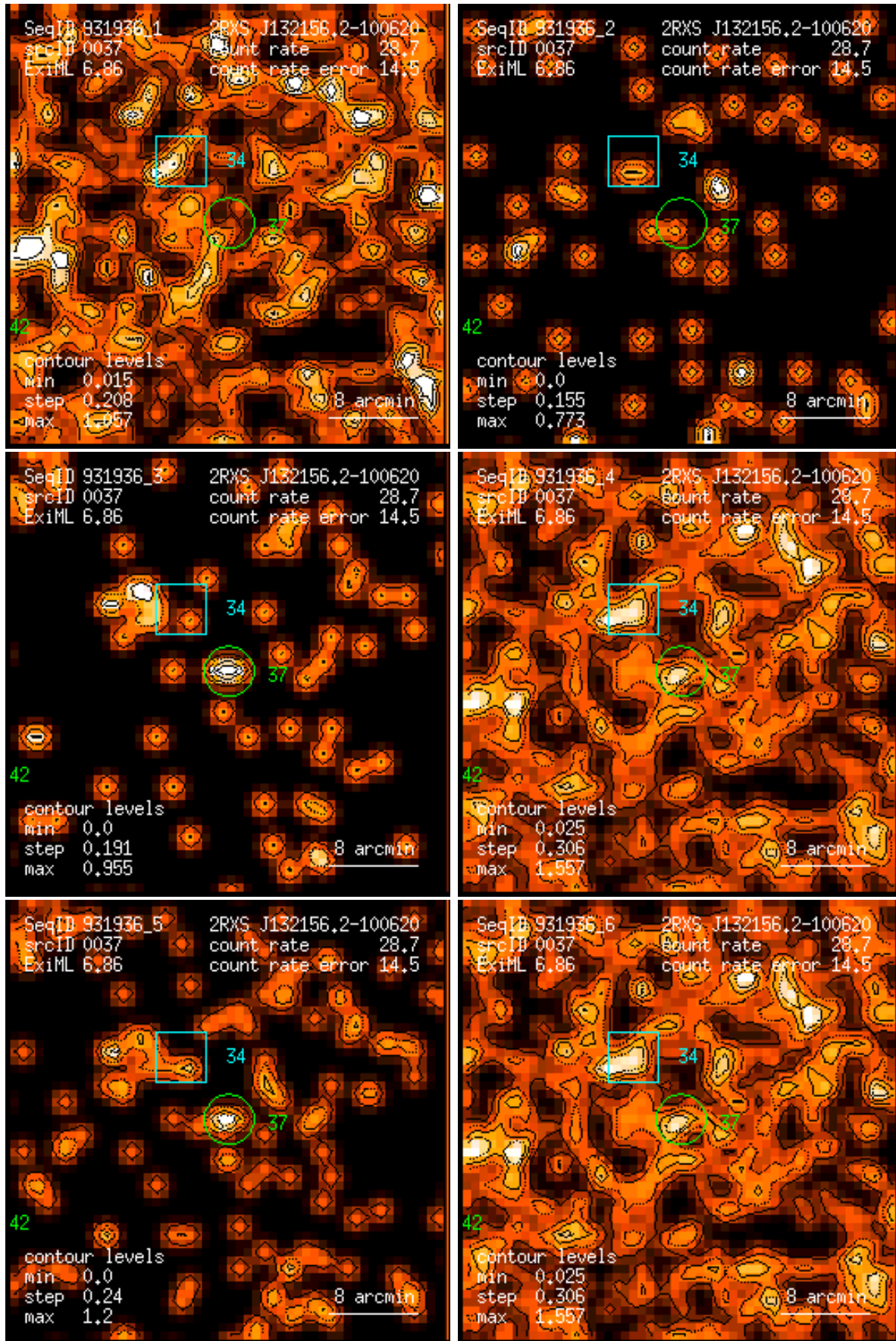
Figure 37: RASS 931936: detection 0037: band rate images, Gaussian filter: (1) PSPC channels 11 – 41, (2) 52 – 90, (3) 91 – 201, (4) 11 – 235, (5) 52 – 201, (6) 11 – 201. Broad band rates in counts/ks. Band rate contour levels in counts/ks/arcmin 2 .
