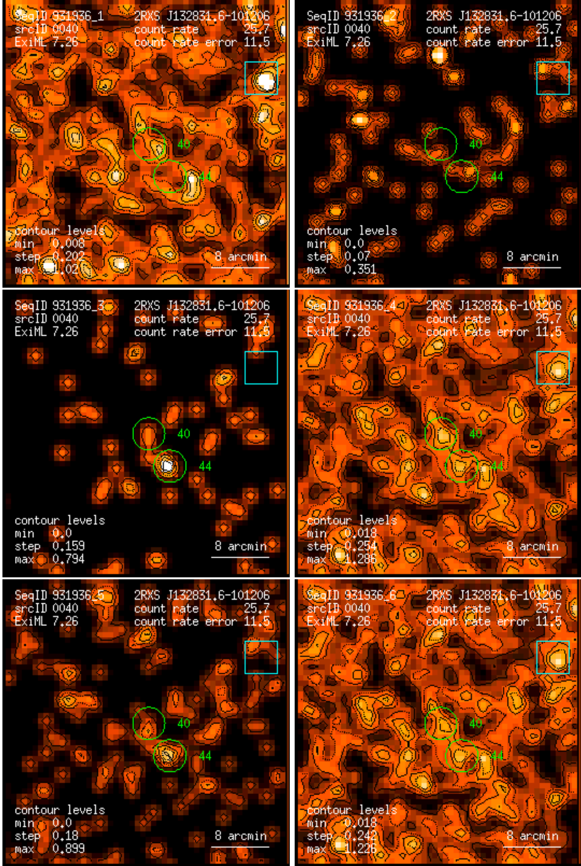
Figure 40: RASS 931936: detection 0040: band rate images, Gaussian filter: (1) PSPC channels 11 – 41, (2) 52 – 90, (3) 91 – 201, (4) 11 – 235, (5) 52 – 201, (6) 11 – 201. Broad band rates in counts/ks. Band rate contour levels in counts/ks/arcmin 2 .
