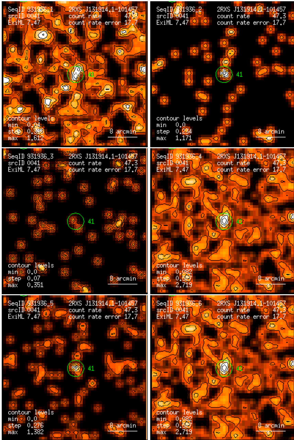
Figure 41: RASS 931936: detection 0041: band rate images, Gaussian filter: (1) PSPC channels 11 – 41, (2) 52 – 90, (3) 91 – 201, (4) 11 – 235, (5) 52 – 201, (6) 11 – 201. Broad band rates in counts/ks. Band rate contour levels in counts/ks/arcmin 2 .
