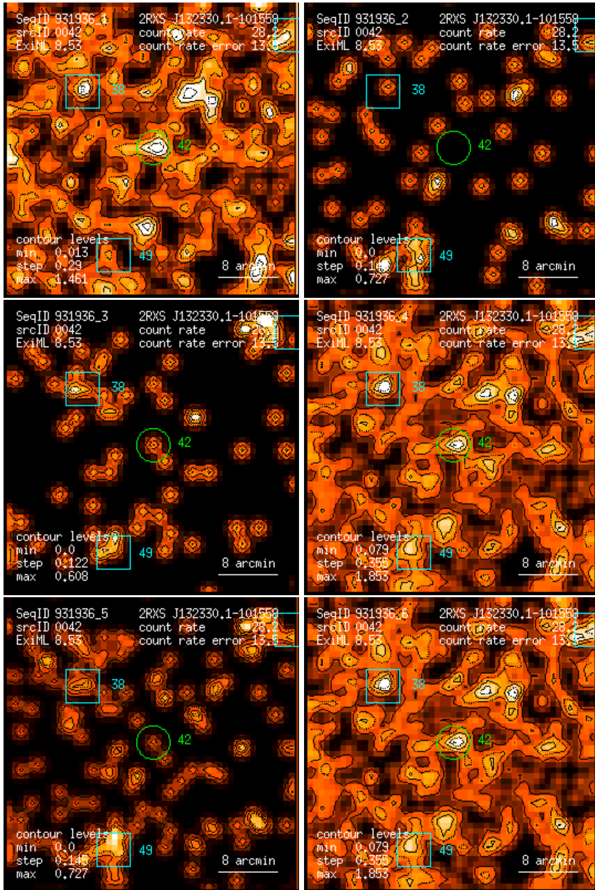
Figure 42: RASS 931936: detection 0042: band rate images, Gaussian filter: (1) PSPC channels 11 – 41, (2) 52 – 90, (3) 91 – 201, (4) 11 – 235, (5) 52 – 201, (6) 11 – 201. Broad band rates in counts/ks. Band rate contour levels in counts/ks/arcmin 2 .
