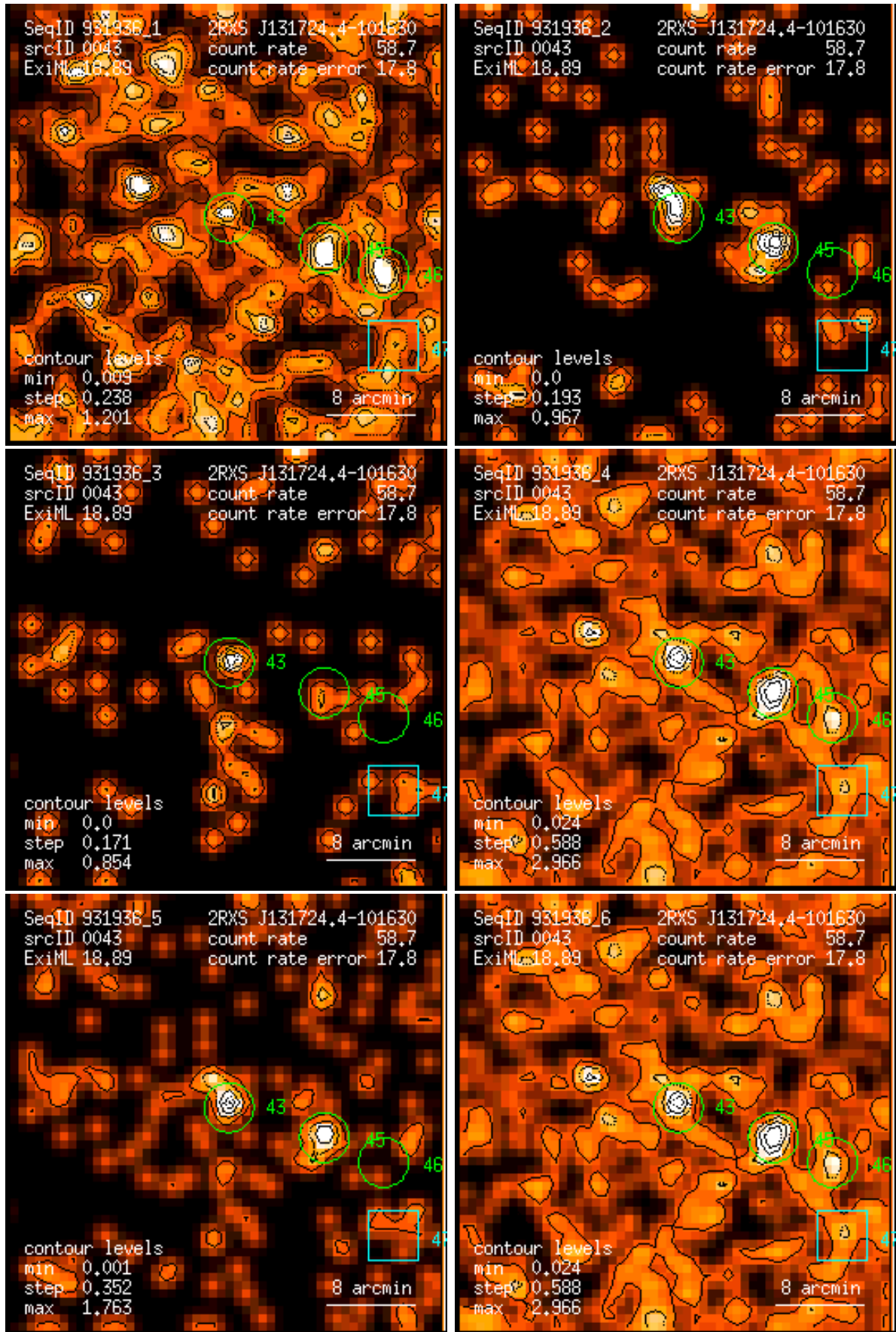
Figure 43: RASS 931936: detection 0043: band rate images, Gaussian filter: (1) PSPC channels 11 – 41, (2) 52 – 90, (3) 91 – 201, (4) 11 – 235, (5) 52 – 201, (6) 11 – 201. Broad band rates in counts/ks. Band rate contour levels in counts/ks/arcmin 2 .
