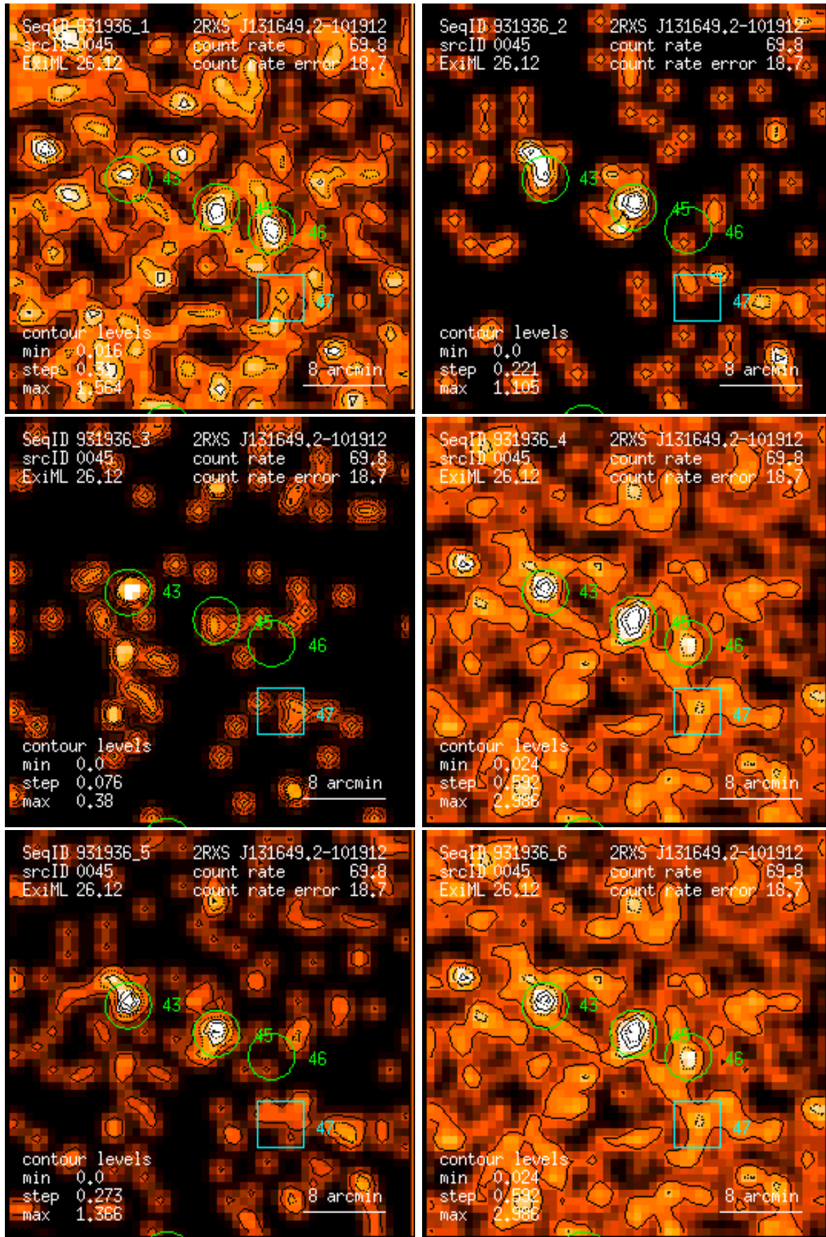
Figure 45: RASS 931936: detection 0045: band rate images, Gaussian filter: (1) PSPC channels 11 – 41, (2) 52 – 90, (3) 91 – 201, (4) 11 – 235, (5) 52 – 201, (6) 11 – 201. Broad band rates in counts/ks. Band rate contour levels in counts/ks/arcmin 2 .
