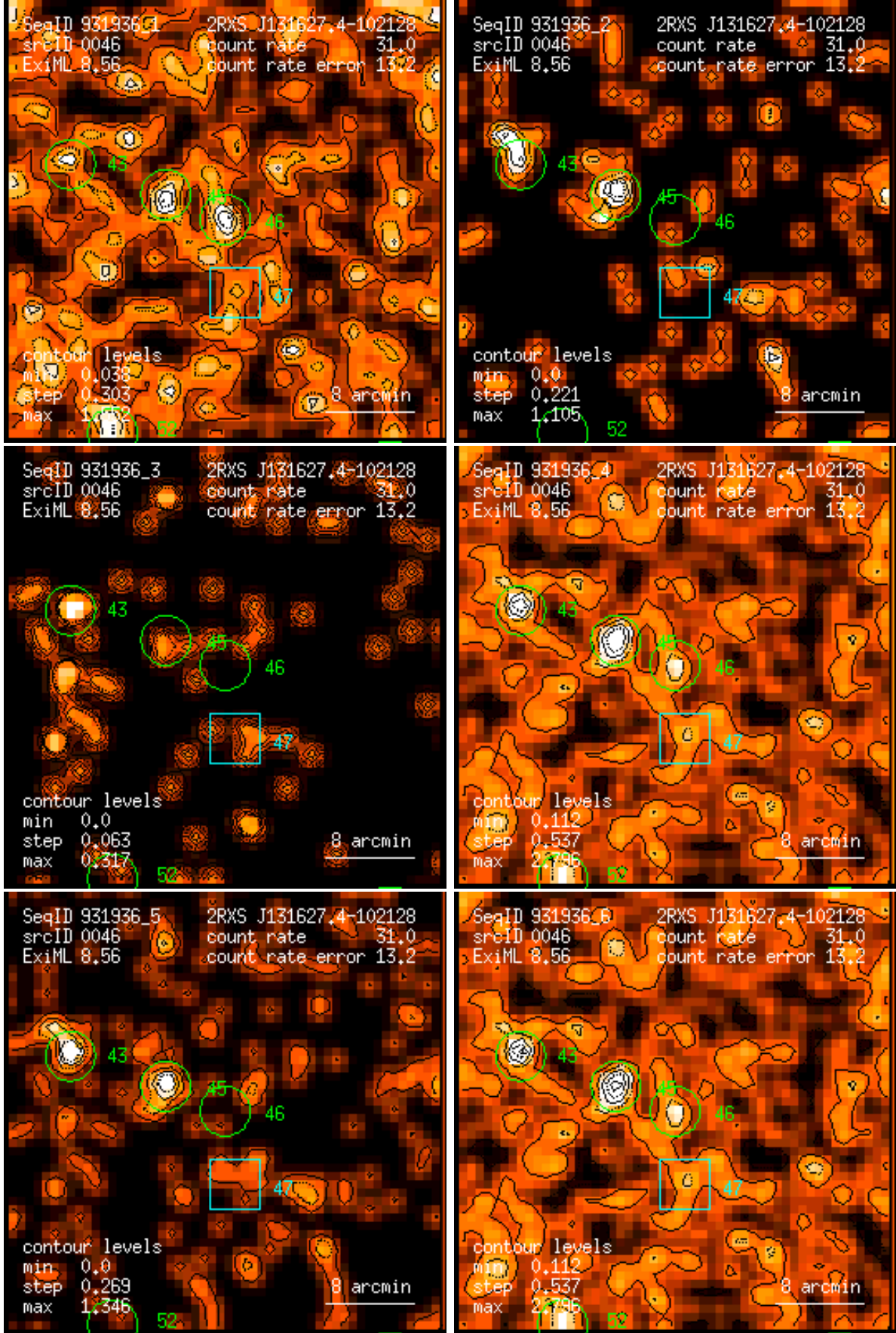
Figure 46: RASS 931936: detection 0046: band rate images, Gaussian filter: (1) PSPC channels 11 – 41, (2) 52 – 90, (3) 91 – 201, (4) 11 – 235, (5) 52 – 201, (6) 11 – 201. Broad band rates in counts/ks. Band rate contour levels in counts/ks/arcmin 2 .
