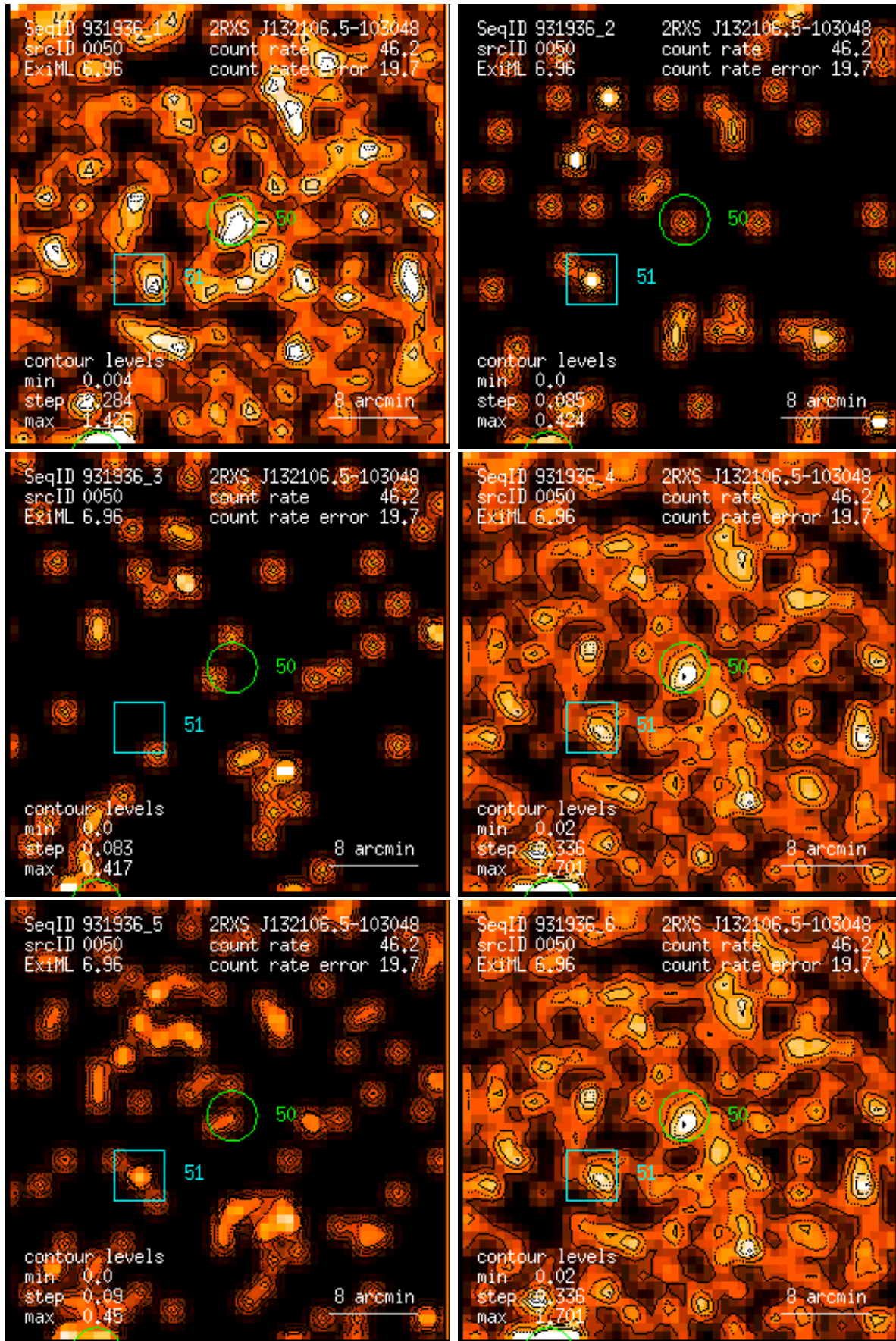
Figure 50: RASS 931936: detection 0050: band rate images, Gaussian filter: (1) PSPC channels 11 – 41, (2) 52 – 90, (3) 91 – 201, (4) 11 – 235, (5) 52 – 201, (6) 11 – 201. Broad band rates in counts/ks. Band rate contour levels in counts/ks/arcmin 2 .
