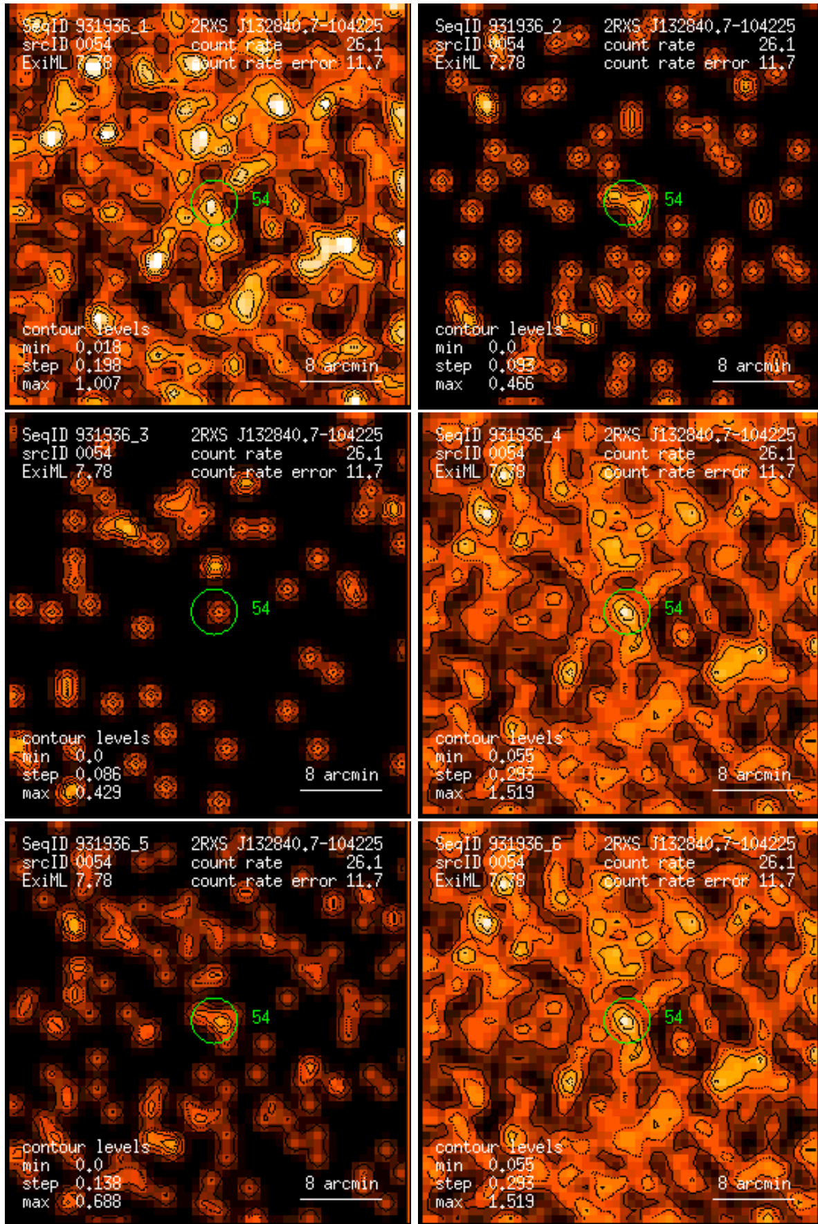
Figure 54: RASS 931936: detection 0054: band rate images, Gaussian filter: (1) PSPC channels 11 – 41, (2) 52 – 90, (3) 91 – 201, (4) 11 – 235, (5) 52 – 201, (6) 11 – 201. Broad band rates in counts/ks. Band rate contour levels in counts/ks/arcmin 2 .
