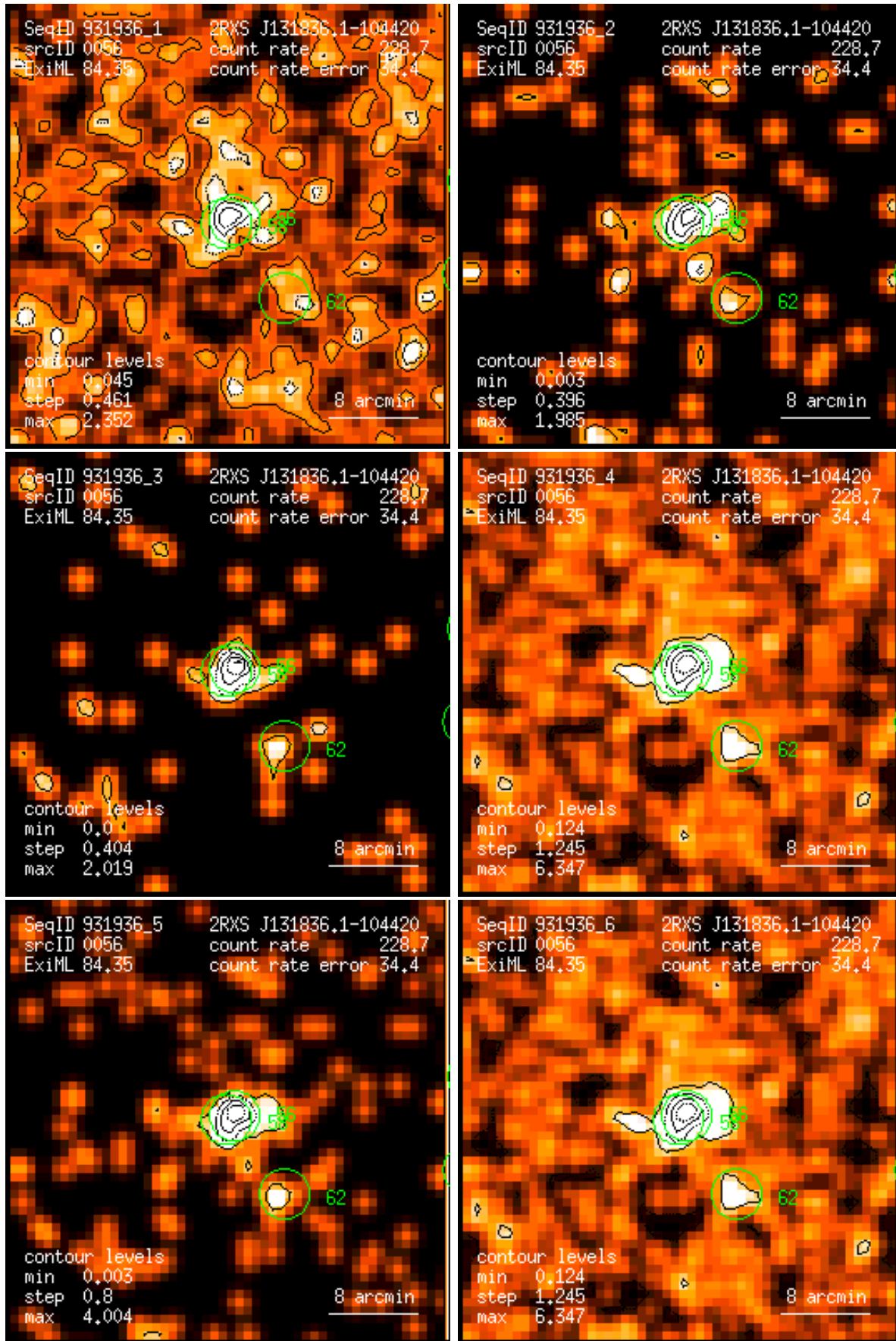
Figure 56: RASS 931936: detection 0056: band rate images, Gaussian filter: (1) PSPC channels 11 – 41, (2) 52 – 90, (3) 91 – 201, (4) 11 – 235, (5) 52 – 201, (6) 11 – 201. Broad band rates in counts/ks. Band rate contour levels in counts/ks/arcmin 2 .
