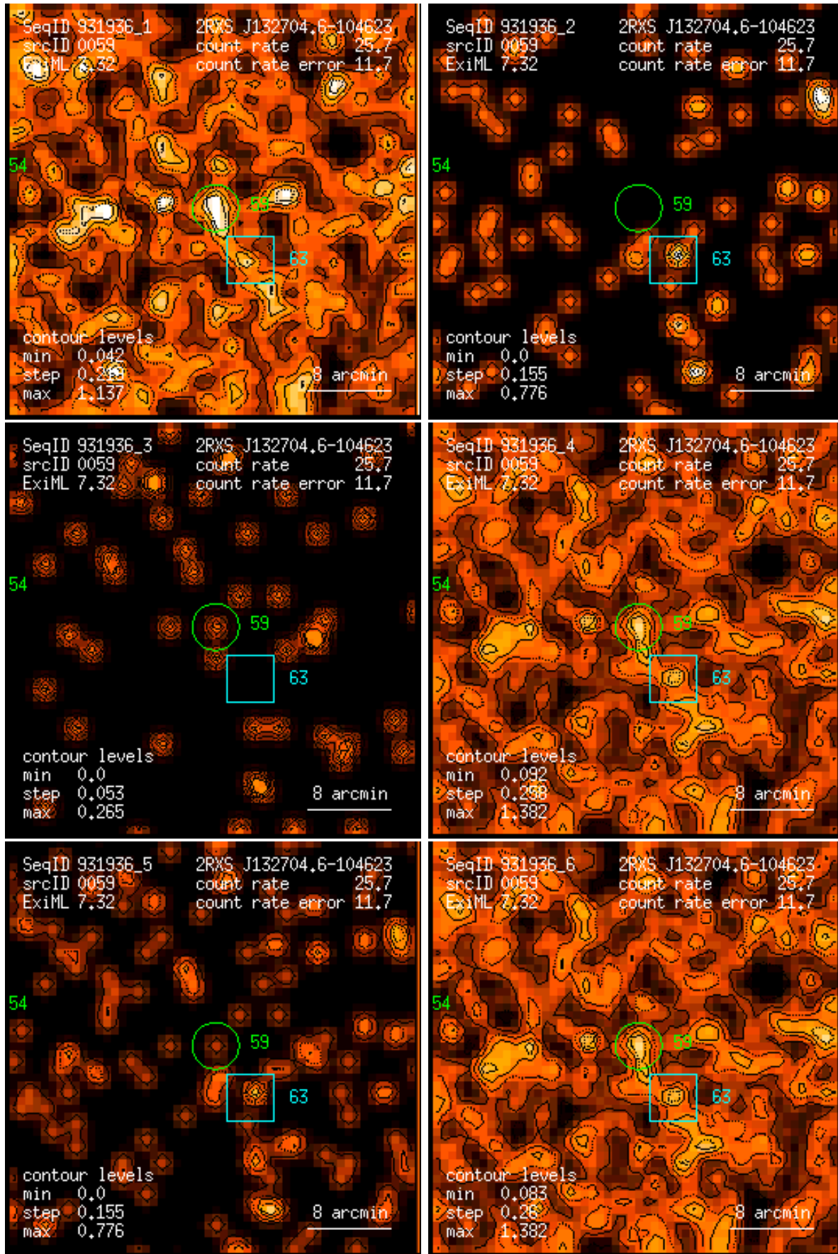
Figure 59: RASS 931936: detection 0059: band rate images, Gaussian filter: (1) PSPC channels 11 – 41, (2) 52 – 90, (3) 91 – 201, (4) 11 – 235, (5) 52 – 201, (6) 11 – 201. Broad band rates in counts/ks. Band rate contour levels in counts/ks/arcmin 2 .
