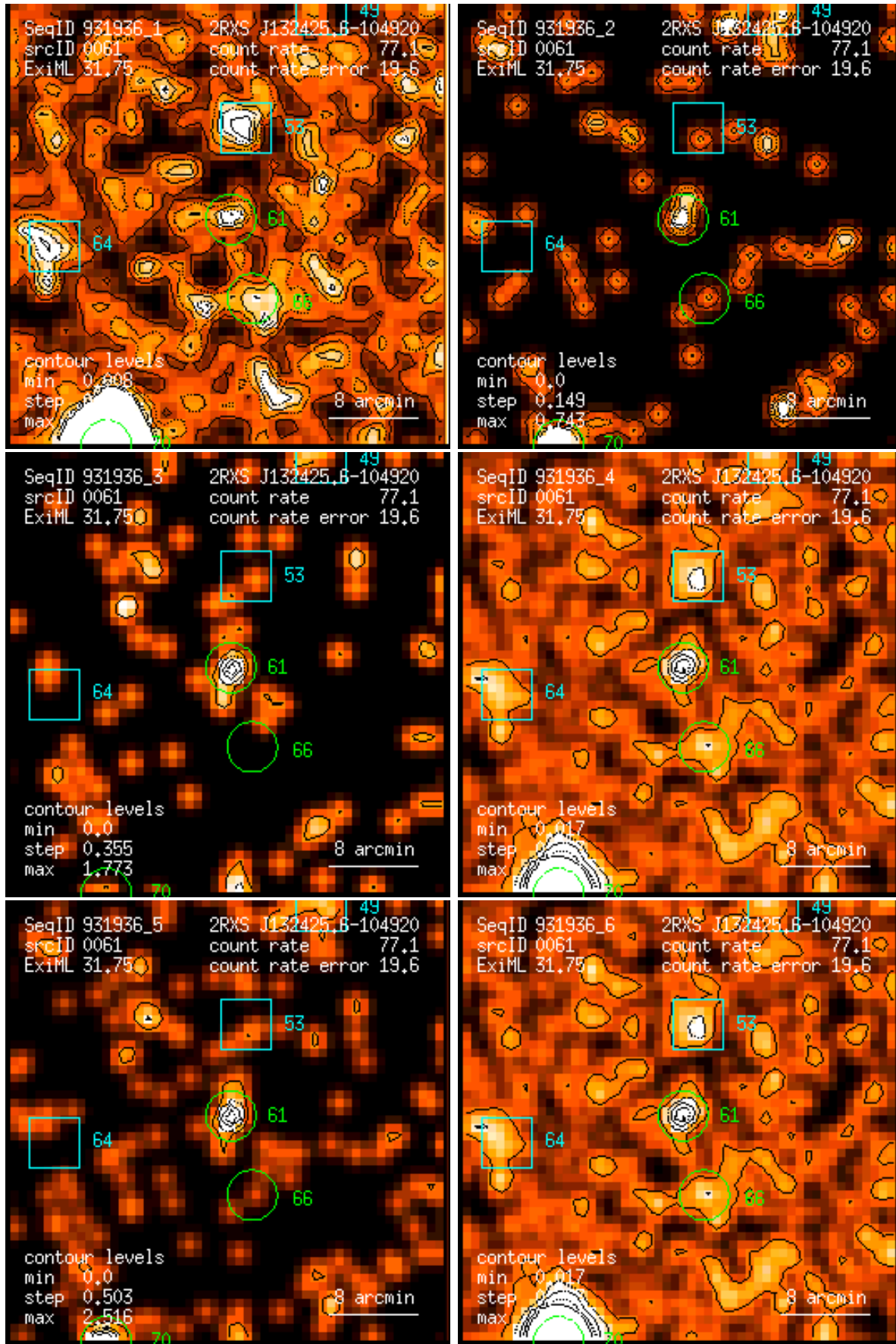
Figure 61: RASS 931936: detection 0061: band rate images, Gaussian filter: (1) PSPC channels 11 – 41, (2) 52 – 90, (3) 91 – 201, (4) 11 – 235, (5) 52 – 201, (6) 11 – 201. Broad band rates in counts/ks. Band rate contour levels in counts/ks/arcmin 2 .
