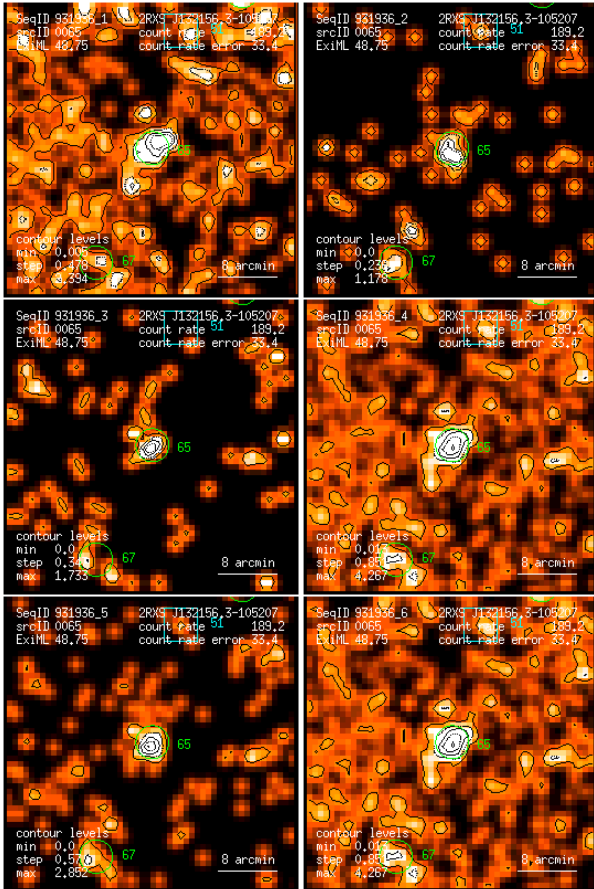
Figure 65: RASS 931936: detection 0065: band rate images, Gaussian filter: (1) PSPC channels 11 – 41, (2) 52 – 90, (3) 91 – 201, (4) 11 – 235, (5) 52 – 201, (6) 11 – 201. Broad band rates in counts/ks. Band rate contour levels in counts/ks/arcmin 2 .
