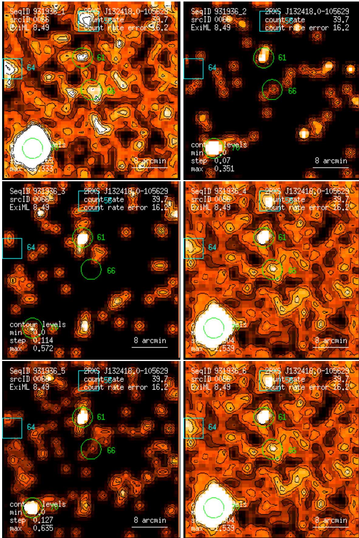
Figure 66: RASS 931936: detection 0066: band rate images, Gaussian filter: (1) PSPC channels 11 – 41, (2) 52 – 90, (3) 91 – 201, (4) 11 – 235, (5) 52 – 201, (6) 11 – 201. Broad band rates in counts/ks. Band rate contour levels in counts/ks/arcmin 2 .
