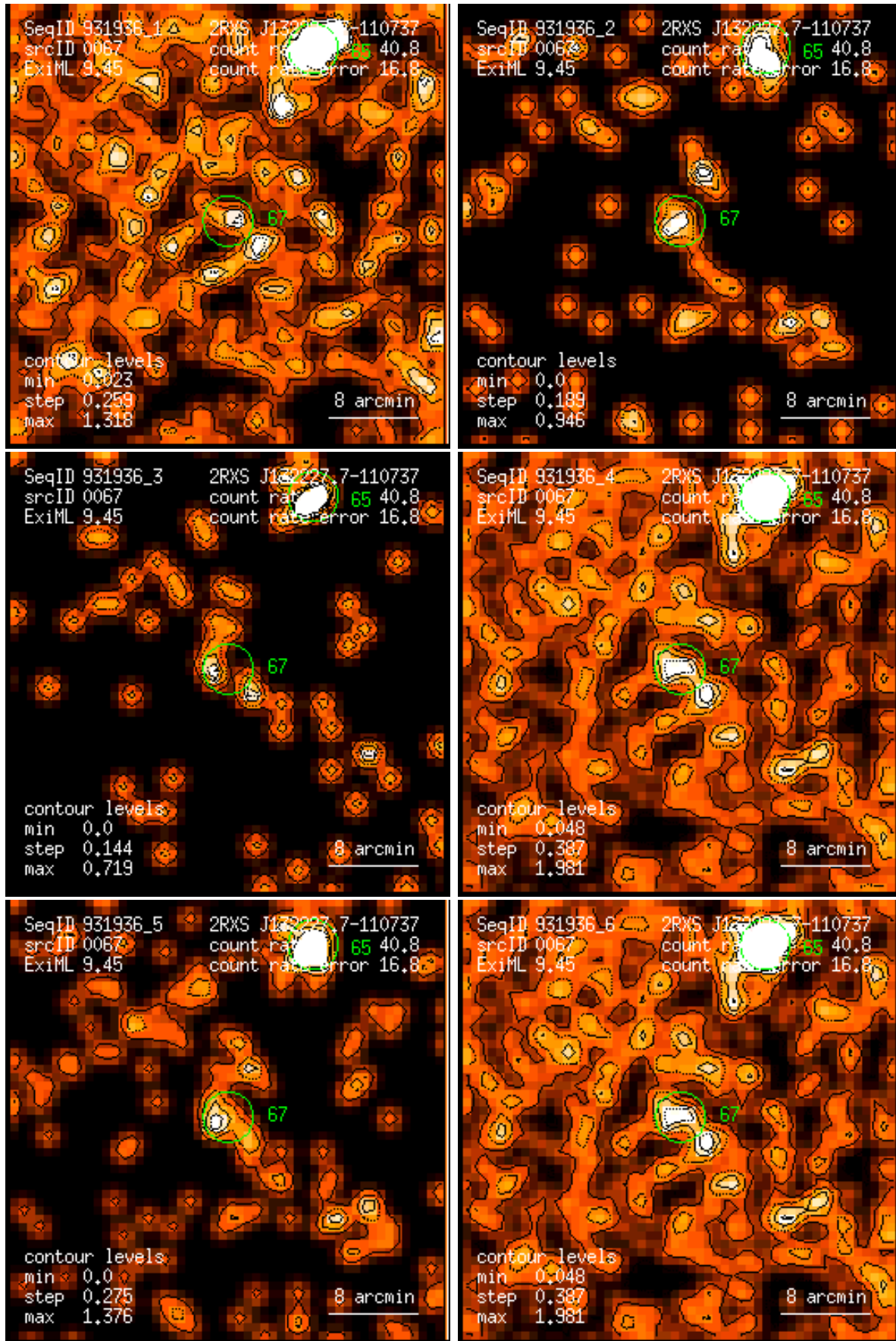
Figure 67: RASS 931936: detection 0067: band rate images, Gaussian filter: (1) PSPC channels 11 – 41, (2) 52 – 90, (3) 91 – 201, (4) 11 – 235, (5) 52 – 201, (6) 11 – 201. Broad band rates in counts/ks. Band rate contour levels in counts/ks/arcmin 2 .
